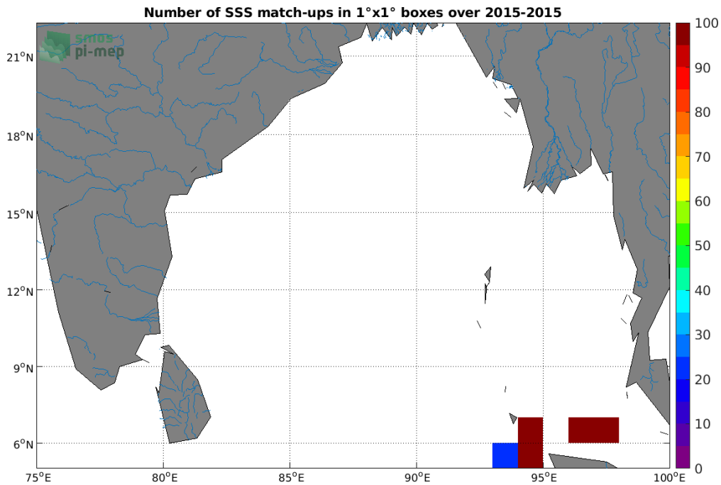
Figure 4: Number of SSS match-ups between TSG (SAMOS) SSS and the SMOS L4 v2 Weekly (CATDS-CECOS-IFREMER) SSS product for the Ganga and Brahmaputra river plumes Pi-MEP region over 1^\circ \times 1^\circ boxes and for the full satellite product period.
