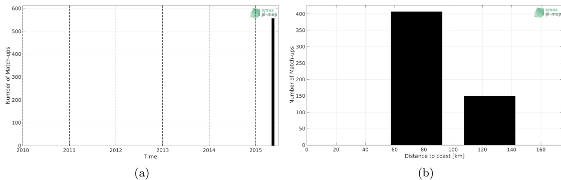
Figure 1: Number of match-ups between TSG (SAMOS) and SMOS L4 v2 Weekly (CATDS-CECOS-IFREMER) SSS as a function of time (a) and as function of the distance to coast (b) over the Ganga and Brahmaputra river plumes Pi-MEP region and for the full satellite product period.
