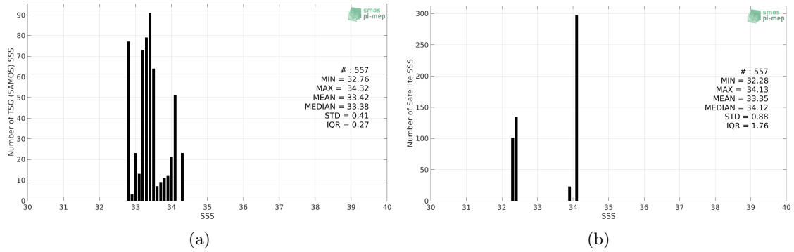
Figure 2: Histograms of SSS from TSG (SAMOS) (a) and SMOS L4 v2 Weekly (CATDS-CECOS-IFREMER) (b) considering all match-up pairs per bins of 0.1 over the Ganga and Brahmaputra river plumes Pi-MEP region and for the full satellite product period.
