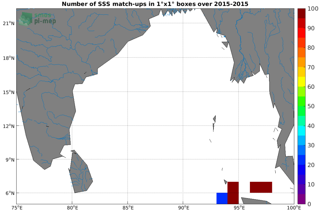
Figure 4: Number of SSS match-ups between TSG (SAMOS) SSS and the SMOS L4 v2 Weekly (CATDS-CECOS-IFREMER) SSS product for the Ganga and Brahmaputra river plumes Pi-MEP region over 1°x1° boxes and for the full satellite product period.
