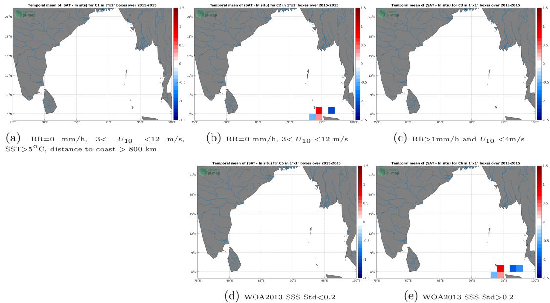
Figure 12: Temporal mean gridded over spatial boxes of size 1^{\circ}\times 1^{\circ} of \Delta\text{SSS} (SMOS-L4-CATDS-CECOS-IFREMER-V2-WEEKLY-0.5DEG - TSG-SAMOS) for 5 different subdatasets corresponding to:RR=0 mm/h, 3 < U_{10} < 12 m/s, SST >5^{\circ}\text{C} , distance to coast > 800 km (a), RR=0 mm/h, 3 < U_{10} < 12 m/s (b), RR >1 mm/h and U_{10} < 4 m/s (c), WOA2013 SSS Std <0.2 (d), WOA2013 SSS Std >0.2 (e).
