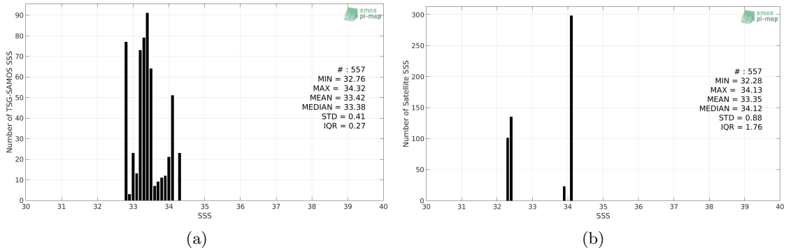
Figure 2: Histograms of SSS from TSG-SAMOS (a) and SMOS-L4-CATDS-CECOS-IFREMER-V2-WEEKLY-0.5DEG (b) considering all match-up pairs per bins of 0.1 over the Ganga and Brahmaputra river plumes Pi-MEP region and for the full satellite product period.
