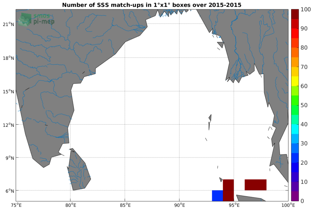
Figure 4: Number of SSS match-ups between TSG-SAMOS SSS and the SMOS-L4-CATDS-CECOS-IFREMER-V2-WEEKLY-0.5DEG SSS product for the Ganga and Brahmaputra river plumes Pi-MEP region over 1°x1° boxes and for the full satellite product period.
