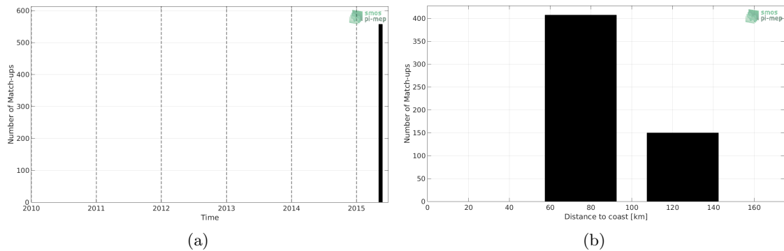
Figure 1: Number of match-ups between TSG-SAMOS and SMOS-L4-CATDS-CECOS-IFREMER-V2-WEEKLY-0.5DEG SSS as a function of time (a) and as function of the distance to coast (b) over the Ganga and Brahmaputra river plumes Pi-MEP region and for the full satellite product period.
