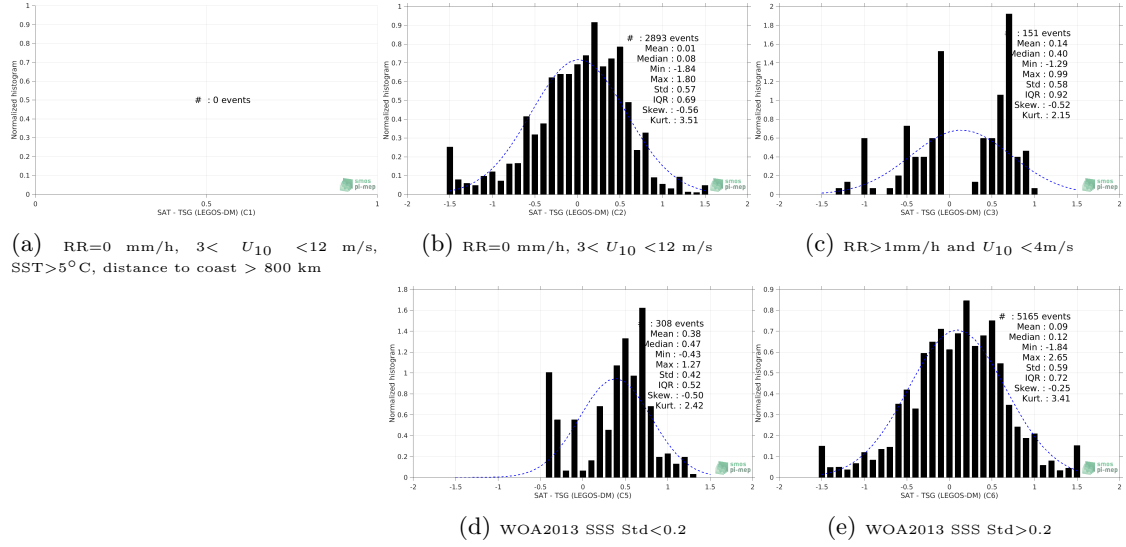
Figure 13: Normalized histogram of \Delta SSS (SMOS L4 v2 Weekly (CATDS-CECOS-IFREMER) - TSG (LEGOS-DM)) for 5 different subdatasets corresponding to: RR=0 mm/h, 3 < U_{10} < 12 m/s, SST>5°C, distance to coast > 800 km (a), RR=0 mm/h, 3 < U_{10} < 12 m/s (b), RR>1mm/h and U_{10} < 4 m/s (c), WOA2013 SSS Std<0.2 (d), WOA2013 SSS Std>0.2 (e).
