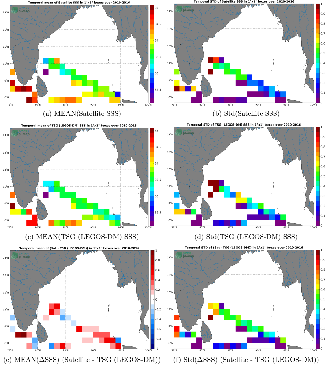
Figure 6: Temporal mean (left) and Std (right) of SSS from SMOS L4 v2 Weekly (CATDS-CECOS-IFREMER) (top), TSG (LEGOS-DM) (middle), and of \Delta SSS (Satellite - TSG (LEGOS-DM)). Only match-up pairs are used to generate these maps.
