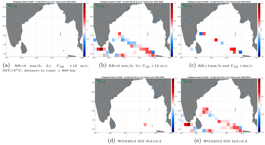
Figure 12: Temporal mean gridded over spatial boxes of size 1^{\circ}\times 1^{\circ} of \Delta\text{SSS} (SMOS L4 v2 Weekly (CATDS-CECOS-IFREMER) - TSG (LEGOS-DM)) for 5 different subdatasets corresponding to:RR=0 mm/h, 3 < U_{10} < 12 m/s, SST >5^{\circ}\text{C} , distance to coast > 800 km (a), RR=0 mm/h, 3 < U_{10} < 12 m/s (b), RR >1 mm/h and U_{10} < 4 m/s (c), WOA2013 SSS Std <0.2 (d), WOA2013 SSS Std >0.2 (e).
