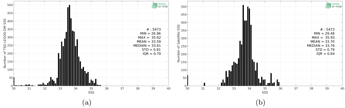
Figure 2: Histograms of SSS from TSG-LEGOS-DM (a) and SMOS-L4-CATDS-CECOS-IFREMER-V2-WEEKLY-0.5DEG (b) considering all match-up pairs per bins of 0.1 over the Ganga and Brahmaputra river plumes Pi-MEP region and for the full satellite product period.
