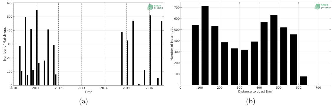
Figure 1: Number of match-ups between TSG-LEGOS-DM and SMOS-L4-CATDS-CECOS-IFREMER-V2-WEEKLY-0.5DEG SSS as a function of time (a) and as function of the distance to coast (b) over the Ganga and Brahmaputra river plumes Pi-MEP region and for the full satellite product period.
