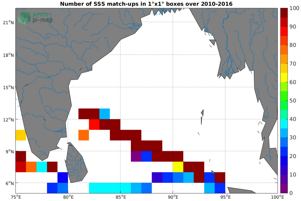
Figure 4: Number of SSS match-ups between TSG-LEGOS-DM SSS and the SMOS-L4-CATDS-CECOS-IFREMER-V2-WEEKLY-0.5DEG SSS product for the Ganga and Brahmaputra river plumes Pi-MEP region over 1^\circ \times 1^\circ boxes and for the full satellite product period.
