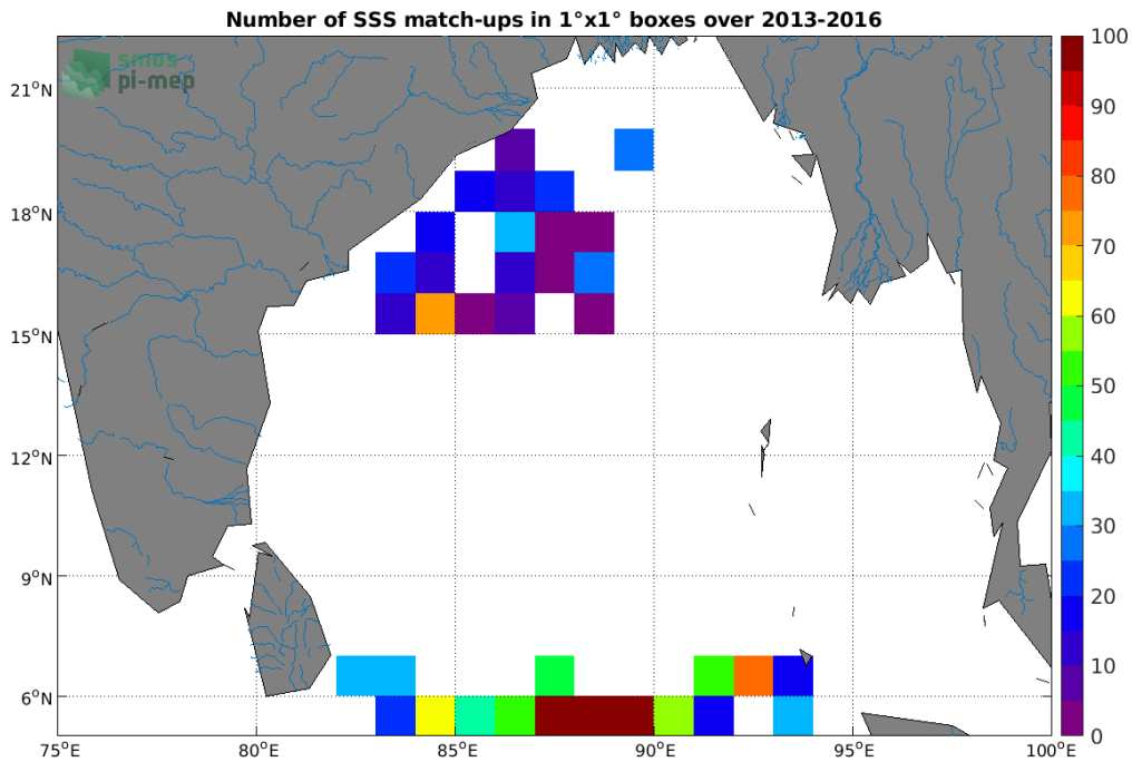
Figure 3: Number of SSS match-ups between Surface drifters SSS and the SMOS L4 v2 Weekly (CATDS-CECOS-IFREMER) SSS product for the Ganga and Brahmaputra river plumes Pi-MEP region over 1^\circ \times 1^\circ boxes and for the full satellite product period.
