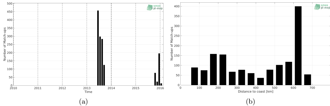
Figure 1: Number of match-ups between Surface drifters and SMOS L4 v2 Weekly (CATDS-CECOS-IFREMER) SSS as a function of time (a) and as function of the distance to coast (b) over the Ganga and Brahmaputra river plumes Pi-MEP region and for the full satellite product period.
