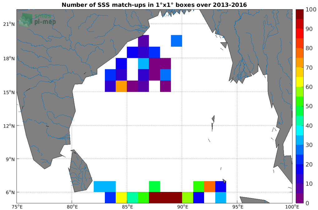
Figure 3: Number of SSS match-ups between Surface drifters SSS and the SMOS L4 v2 Weekly (CATDS-CECOS-IFREMER) SSS product for the Ganga and Brahmaputra river plumes Pi-MEP region over 1°x1° boxes and for the full satellite product period.
