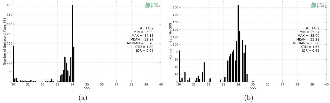
Figure 2: Histograms of SSS from Surface drifters (a) and SMOS L4 v2 Weekly (CATDS-CECOS-IFREMER) (b) considering all match-up pairs per bins of 0.1 over the Ganga and Brahmaputra river plumes Pi-MEP region and for the full satellite product period.
