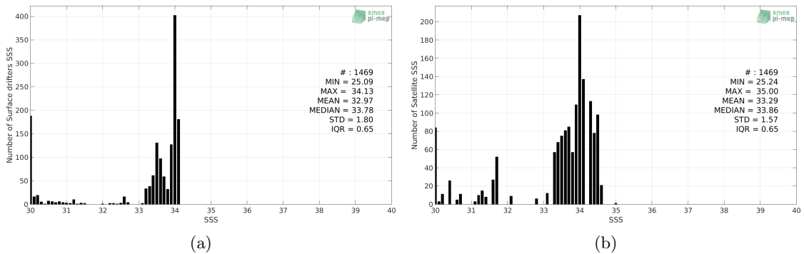
Figure 2: Histograms of SSS from Surface drifters (a) and SMOS-L4-CATDS-CECOS-IFREMER-V2-WEEKLY-0.5DEG (b) considering all match-up pairs per bins of 0.1 over the Ganga and Brahmaputra river plumes Pi-MEP region and for the full satellite product period.
