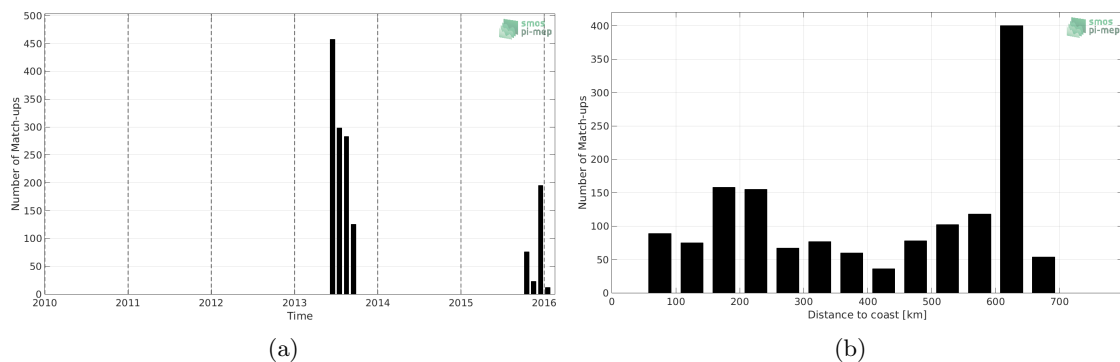
Figure 1: Number of match-ups between Surface drifters and SMOS-L4-CATDS-CECOS-IFREMER-V2-WEEKLY-0.5DEG SSS as a function of time (a) and as function of the distance to coast (b) over the Ganga and Brahmaputra river plumes Pi-MEP region and for the full satellite product period.
