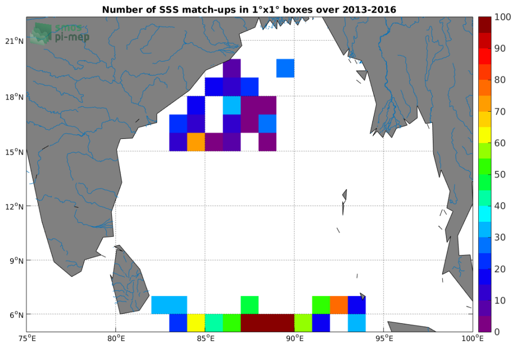
Figure 3: Number of SSS match-ups between Surface drifters SSS and the SMOS-L4-CATDS-CECOS-IFREMER-V2-WEEKLY-0.5DEG SSS product for the Ganga and Brahmaputra river plumes Pi-MEP region over 1°x1° boxes and for the full satellite product period.
