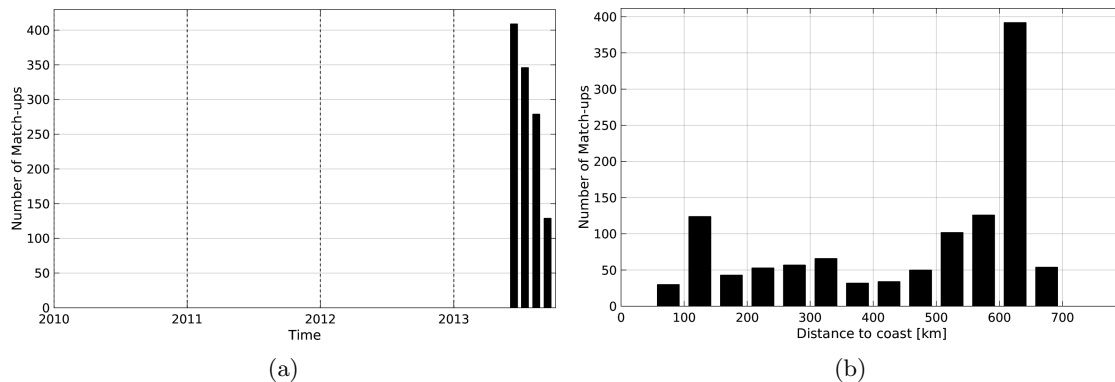
Figure 1: Number of match-ups between Surface drifters and SMOS-L4-CATDS-CECOS-IFREMER-V2-WEEKLY-0.5DEG SSS as a function of time (a) and as function of the distance to coast (b) over the Ganga and Brahmaputra river plumes Pi-MEP region and for the full satellite product period.
