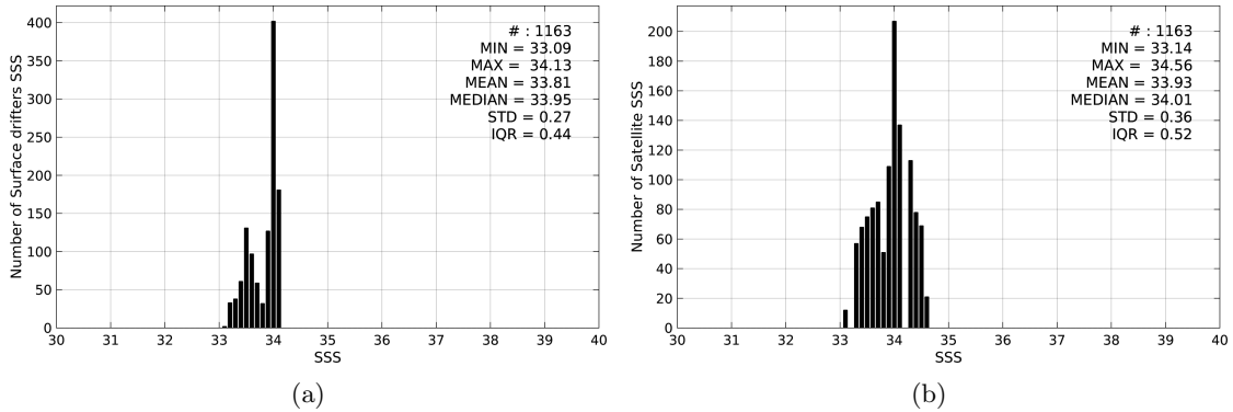
Figure 2: Histograms of SSS from Surface drifters (a) and SMOS-L4-CATDS-CECOS-IFREMER-V2-WEEKLY-0.5DEG (b) considering all match-up pairs per bins of 0.1 over the Ganga and Brahmaputra river plumes Pi-MEP region and for the full satellite product period.
