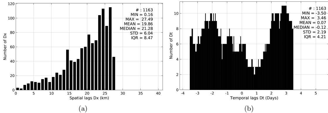
Figure 4: Histograms of the spatial (a) and temporal (b) lags between the time of the Surface drifters measurements and the date of the corresponding SMOS-L4-CATDS-CECOS-IFREMER-V2-WEEKLY-0.5DEG SSS product.
