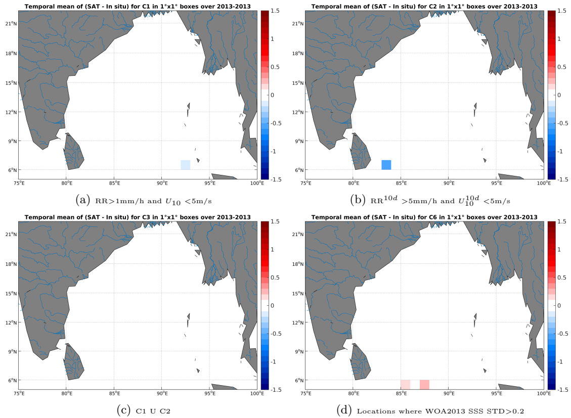
Figure 11: Temporal mean gridded over spatial boxes of size 1°x1° of \Delta SSS (SMOS-L4-CATDS-CECOS-IFREMER-V2-WEEKLY-0.5DEG - Surface drifters) for 4 different subdatasets corresponding to:RR>1mm/h and U_{10} < 5\text{m/s} (a), RR^{10d} > 5\text{mm/h} and U_{10}^{10d} < 5\text{m/s} (b), C1 U C2 (c),Locations where WOA2013 SSS STD>0.2 (d).
