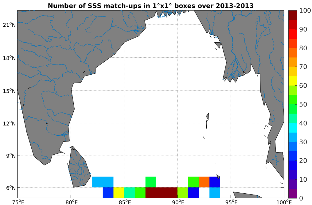
Figure 3: Number of SSS match-ups between Surface drifters SSS and the SMOS-L4-CATDS-CECOS-IFREMER-V2-WEEKLY-0.5DEG SSS product for the Ganga and Brahmaputra river plumes Pi-MEP region over 1^\circ \times 1^\circ boxes and for the full satellite product period.
