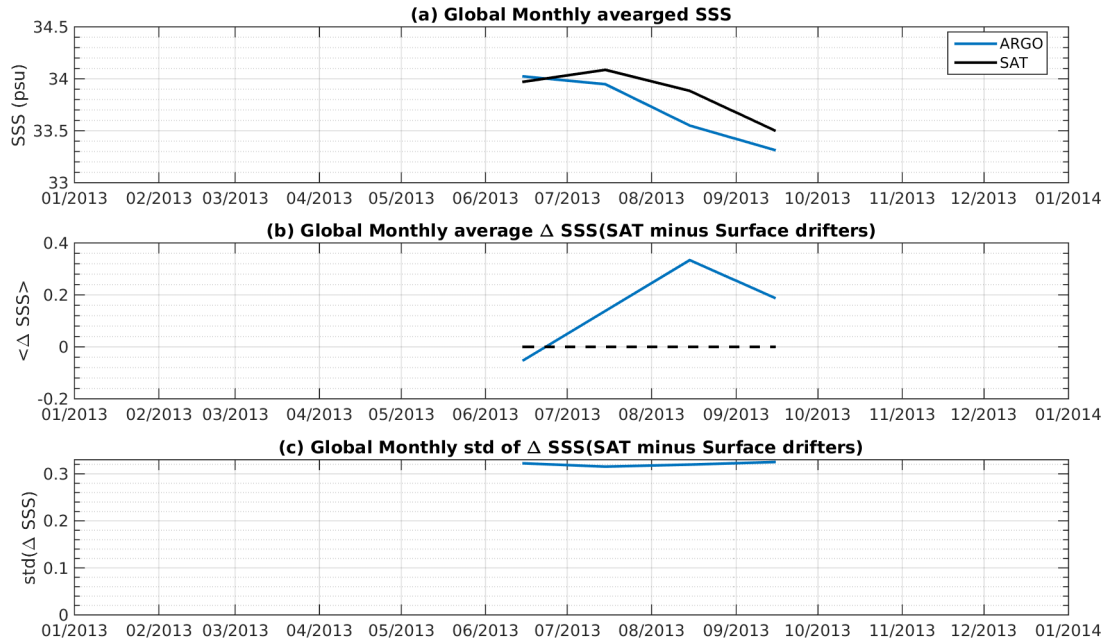
Figure 6: Time series of the monthly averaged mean SSS (top), mean \Delta SSS (Satellite - Surface drifters) and STD of \Delta SSS (Satellite - Surface drifters) over the Ganga and Brahmaputra river plumes Pi-MEP region considering all match-ups collected by the Pi-MEP platform.
