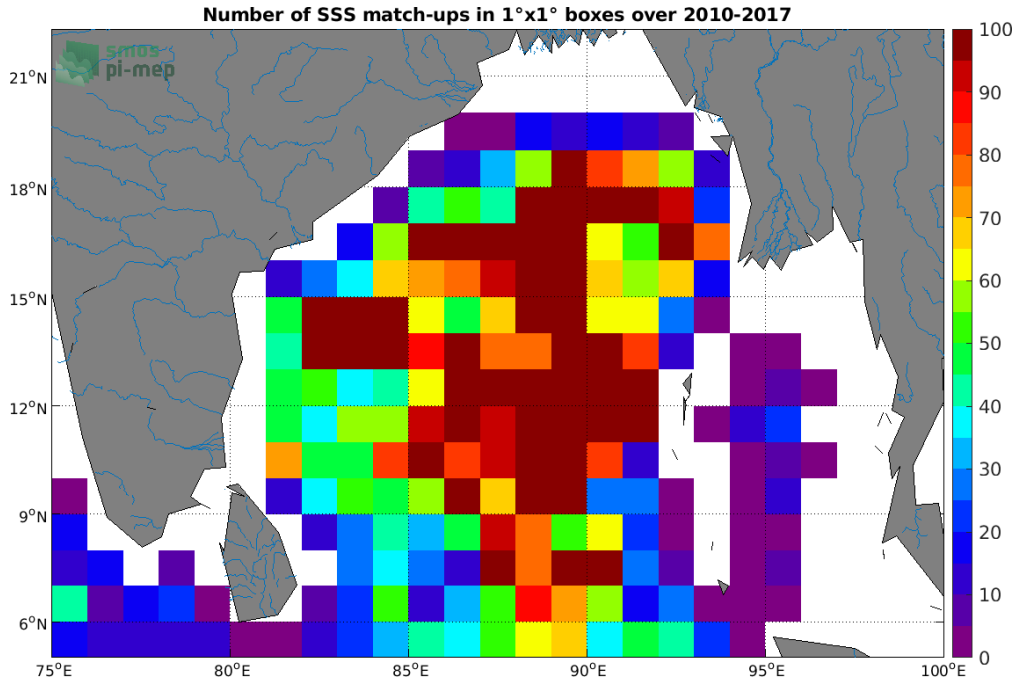
Figure 4: Number of SSS match-ups between Argo SSS and the SMOS L4 v2 Weekly (CATDS-CECOS-IFREMER) SSS product for the Ganga and Brahmaputra river plumes Pi-MEP region over 1^\circ \times 1^\circ boxes and for the full satellite product period.
