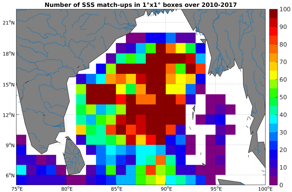
Figure 4: Number of SSS match-ups between Argo SSS and the SMOS-L4-CATDS-CECOS-IFREMER-V2-WEEKLY-0.5DEG SSS product for the Ganga and Brahmaputra river plumes Pi-MEP region over 1^\circ \times 1^\circ boxes and for the full satellite product period.
