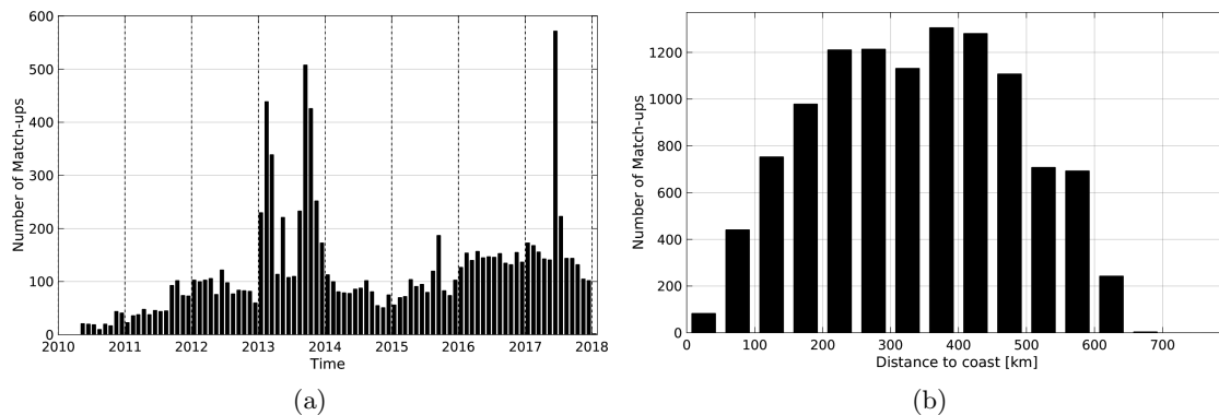
Figure 1: Number of match-ups between Argo and SMOS-L4-CATDS-CECOS-IFREMER-V2-WEEKLY-0.5DEG SSS as a function of time (a) and as function of the distance to coast (b) over the Ganga and Brahmaputra river plumes Pi-MEP region and for the full satellite product period.
