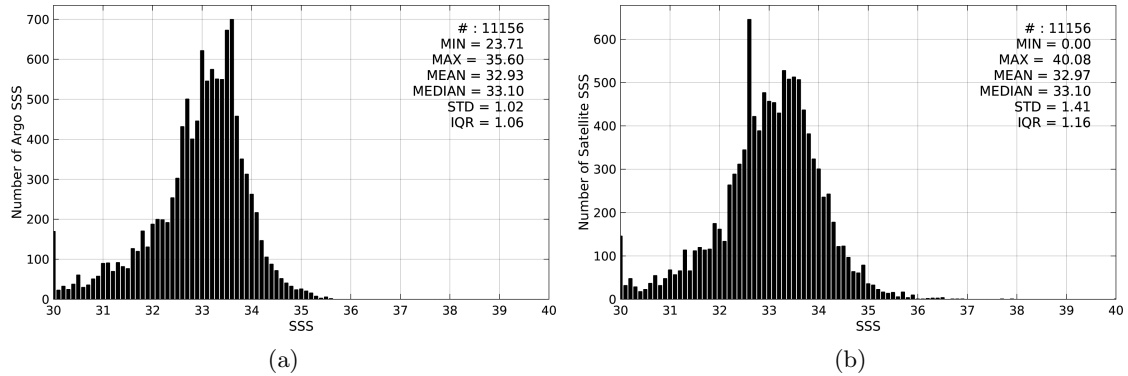
Figure 2: Histograms of SSS from Argo (a) and SMOS-L4-CATDS-CECOS-IFREMER-V2-WEEKLY-0.5DEG (b) considering all match-up pairs per bins of 0.1 over the Ganga and Brahmaputra river plumes Pi-MEP region and for the full satellite product period.
