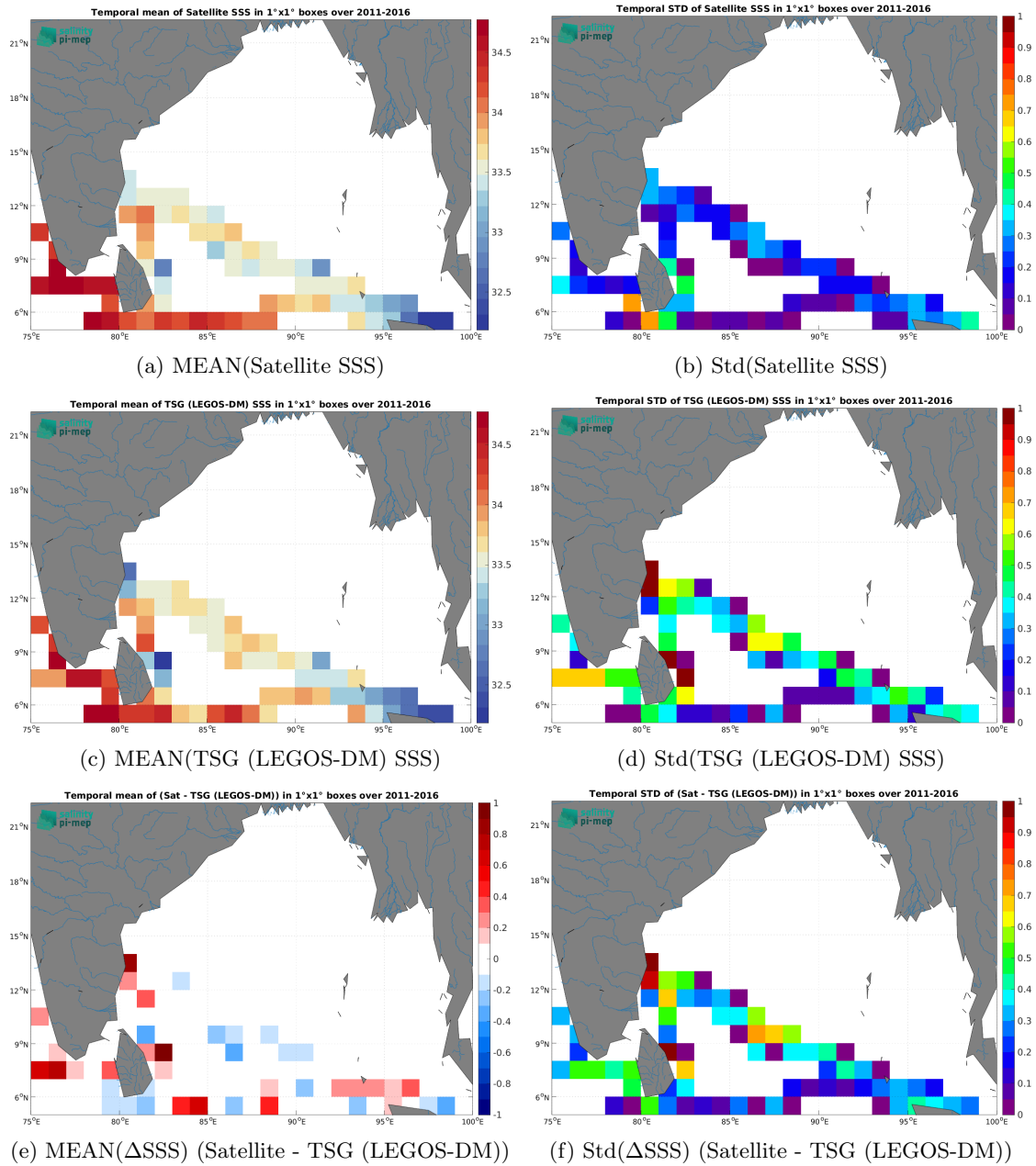
Figure 7: Temporal mean (left) and Std (right) of SSS from SMOS SSS L4 v2 - Daily (BEC) (top), TSG (LEGOS-DM) (middle), and of \Delta SSS (Satellite - TSG (LEGOS-DM)). Only match-up pairs are used to generate these maps.
