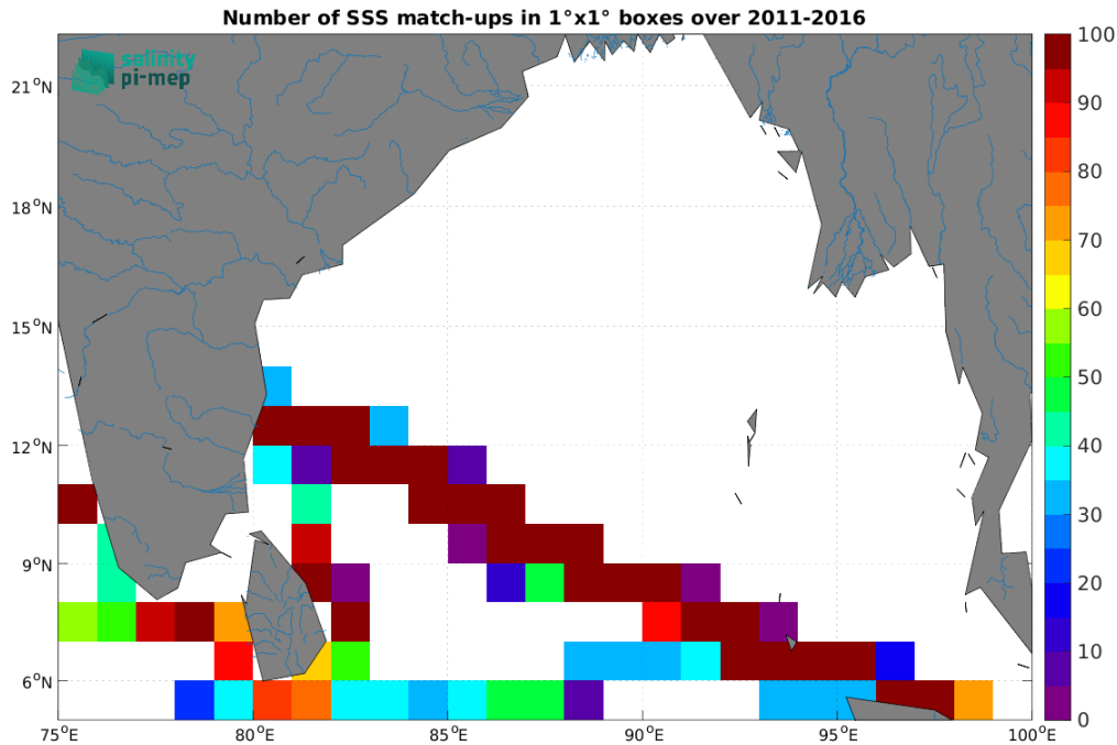
Figure 5: Number of SSS match-ups between TSG (LEGOS-DM) SSS and the SMOS SSS L4 v2 - Daily (BEC) SSS product for the Ganga and Brahmaputra river plumes Pi-MEP region over 1°×1° boxes and for the full satellite product period.
