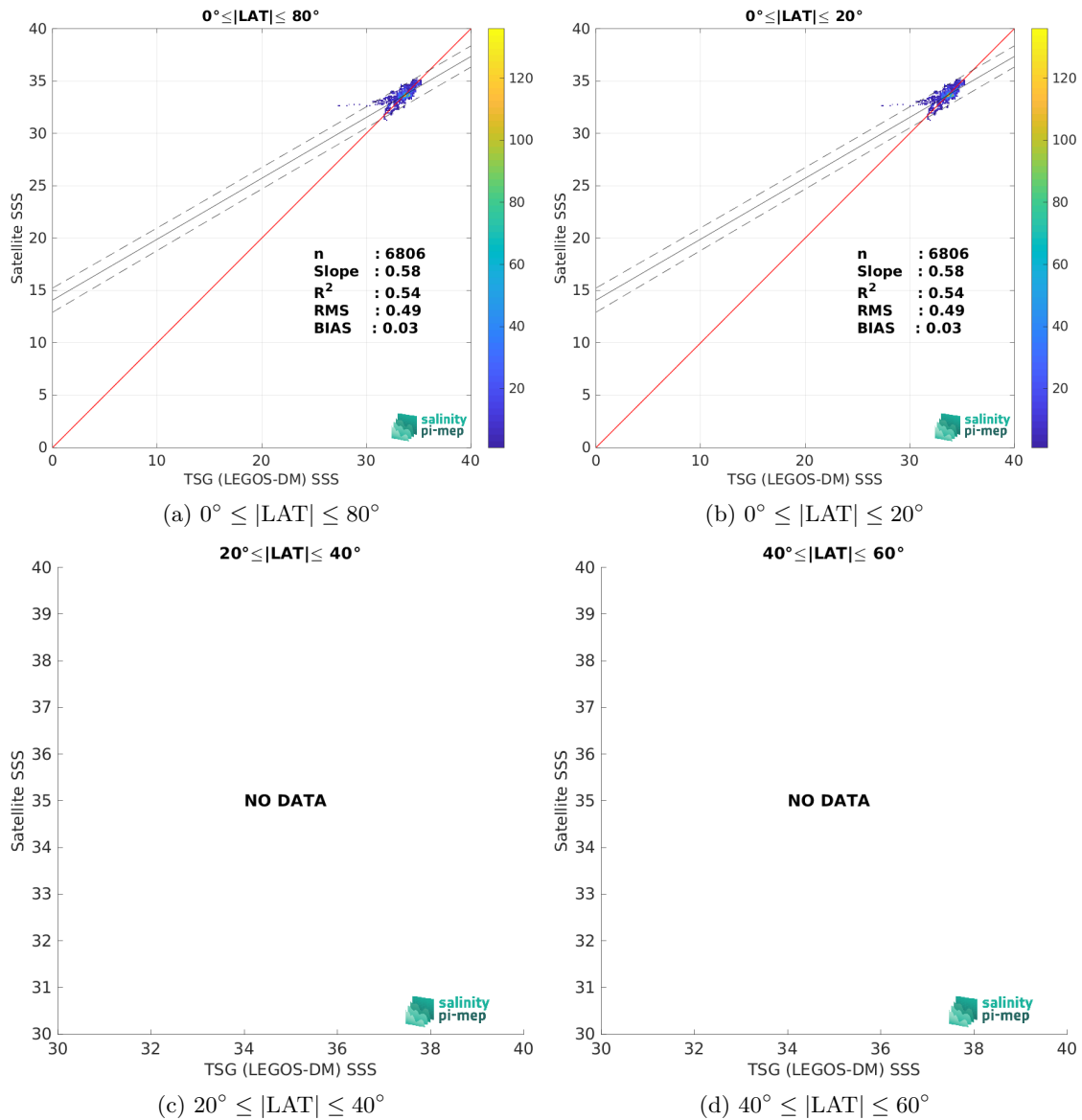
Figure 10: Contour maps of the concentration of SMOS SSS L4 v2 - Daily (BEC) SSS (y-axis) versus TSG (LEGOS-DM) SSS (x-axis) at match-up pairs for different latitude bands. For each plot, the red line shows x=y . The black thin and dashed lines indicate a linear fit through the data cloud and the \pm 95\% confidence levels, respectively. The number match-up pairs n , the slope and R^2 coefficient of the linear fit, the root mean square (RMS) and the mean bias between satellite and in situ data are indicated for each latitude band in each plots.
