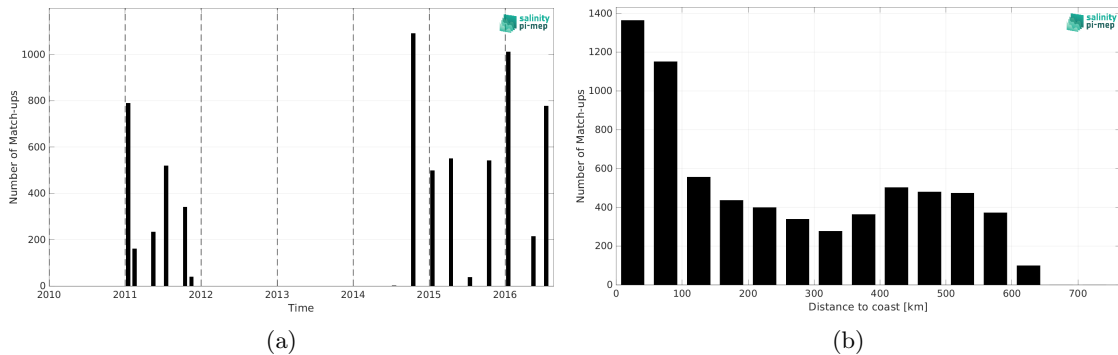
Figure 2: Number of match-ups between TSG (LEGOS-DM) and SMOS SSS L4 v2 - Daily (BEC) SSS as a function of time (a) and as function of the distance to coast (b) over the Ganga and Brahmaputra river plumes Pi-MEP region and for the full satellite product period.
