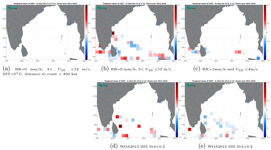
Figure 14: Temporal mean gridded over spatial boxes of size 1^\circ \times 1^\circ of \Delta SSS (SMOS SSS L4 v2 - Daily (BEC) - TSG (LEGOS-DM)) for 5 different subdatasets corresponding to:RR=0 mm/h, 3 < U_{10} < 12 m/s, SST>5°C, distance to coast > 800 km (a), RR=0 mm/h, 3 < U_{10} < 12 m/s (b), RR>1mm/h and U_{10} < 4 m/s (c), WOA2013 SSS Std<0.2 (d), WOA2013 SSS Std>0.2 (e).
