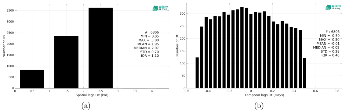
Figure 6: Histograms of the spatial (a) and temporal (b) lags between the location/time of the TSG (LEGOS-DM) measurement and the date of the corresponding SMOS SSS L4 v2 - Daily (BEC) SSS pixel.
