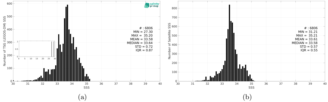
Figure 3: Histograms of SSS from TSG (LEGOS-DM) (a) and SMOS SSS L4 v2 - Daily (BEC) (b) considering all match-up pairs per bins of 0.1 over the Ganga and Brahmaputra river plumes Pi-MEP region and for the full satellite product period.
