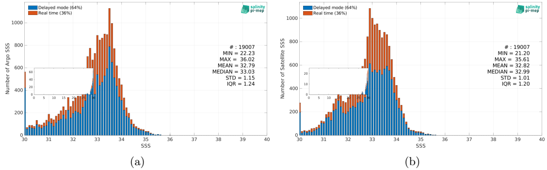
Figure 3: Histograms of SSS from Argo (a) and SMOS SSS L4 v2 - Daily (BEC) (b) considering all match-up pairs per bins of 0.1 over the Ganga and Brahmaputra river plumes Pi-MEP region and for the full satellite product period.
