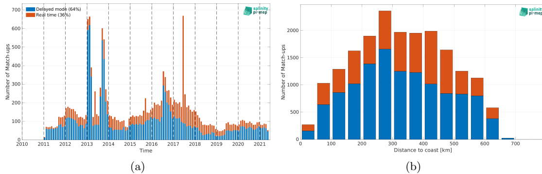
Figure 2: Number of match-ups between Argo and SMOS SSS L4 v2 - Daily (BEC) SSS as a function of time (a) and as function of the distance to coast (b) over the Ganga and Brahmaputra river plumes Pi-MEP region and for the full satellite product period.
