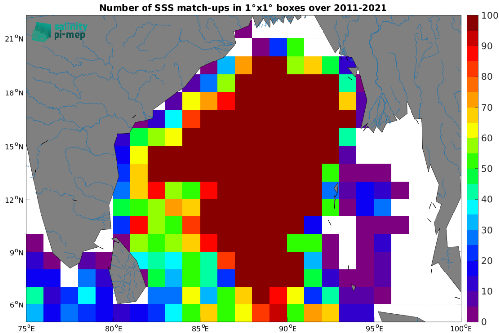
Figure 5: Number of SSS match-ups between Argo SSS and the SMOS SSS L4 v2 - Daily (BEC) SSS product for the Ganga and Brahmaputra river plumes Pi-MEP region over 1^{\circ} \times 1^{\circ} boxes and for the full satellite product period.
