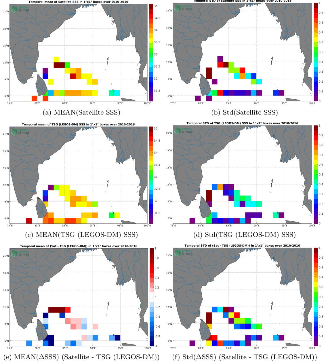
Figure 6: Temporal mean (left) and Std (right) of SSS from SMOS SSS L3 v3 Monthly (ICDC) (top), TSG (LEGOS-DM) (middle), and of \Delta SSS (Satellite - TSG (LEGOS-DM)). Only match-up pairs are used to generate these maps.
