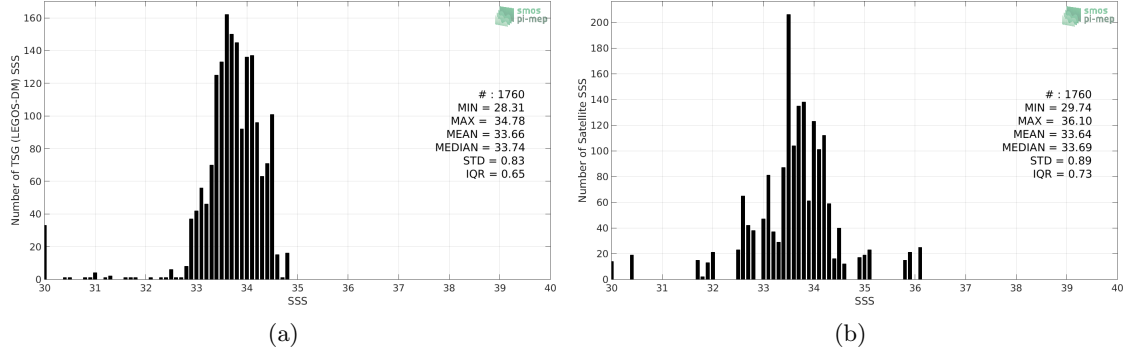
Figure 2: Histograms of SSS from TSG (LEGOS-DM) (a) and SMOS SSS L3 v3 Monthly (ICDC) (b) considering all match-up pairs per bins of 0.1 over the Ganga and Brahmaputra river plumes Pi-MEP region and for the full satellite product period.
