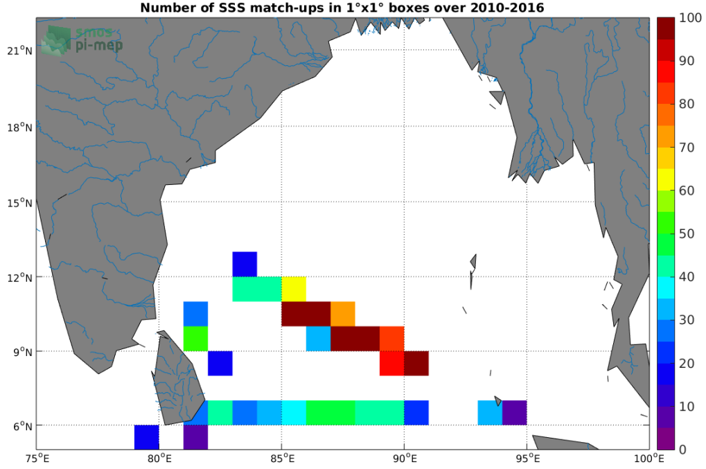
Figure 4: Number of SSS match-ups between TSG (LEGOS-DM) SSS and the SMOS SSS L3 v3 Monthly (ICDC) SSS product for the Ganga and Brahmaputra river plumes Pi-MEP region over 1^\circ \times 1^\circ boxes and for the full satellite product period.
