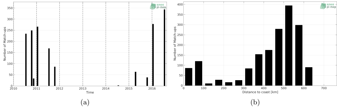
Figure 1: Number of match-ups between TSG (LEGOS-DM) and SMOS SSS L3 v3 Monthly (ICDC) SSS as a function of time (a) and as function of the distance to coast (b) over the Ganga and Brahmaputra river plumes Pi-MEP region and for the full satellite product period.
