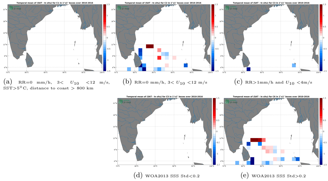
Figure 12: Temporal mean gridded over spatial boxes of size 1^\circ \times 1^\circ of \Delta SSS (SMOS SSS L3 v3 Monthly (ICDC) - TSG (LEGOS-DM)) for 5 different subdatasets corresponding to: RR=0 mm/h, 3 < U_{10} < 12 m/s, SST >5^\circ\text{C} , distance to coast > 800 km (a), RR=0 mm/h, 3 < U_{10} < 12 m/s (b), RR >1 mm/h and U_{10} < 4 m/s (c), WOA2013 SSS Std <0.2 (d), WOA2013 SSS Std >0.2 (e).
