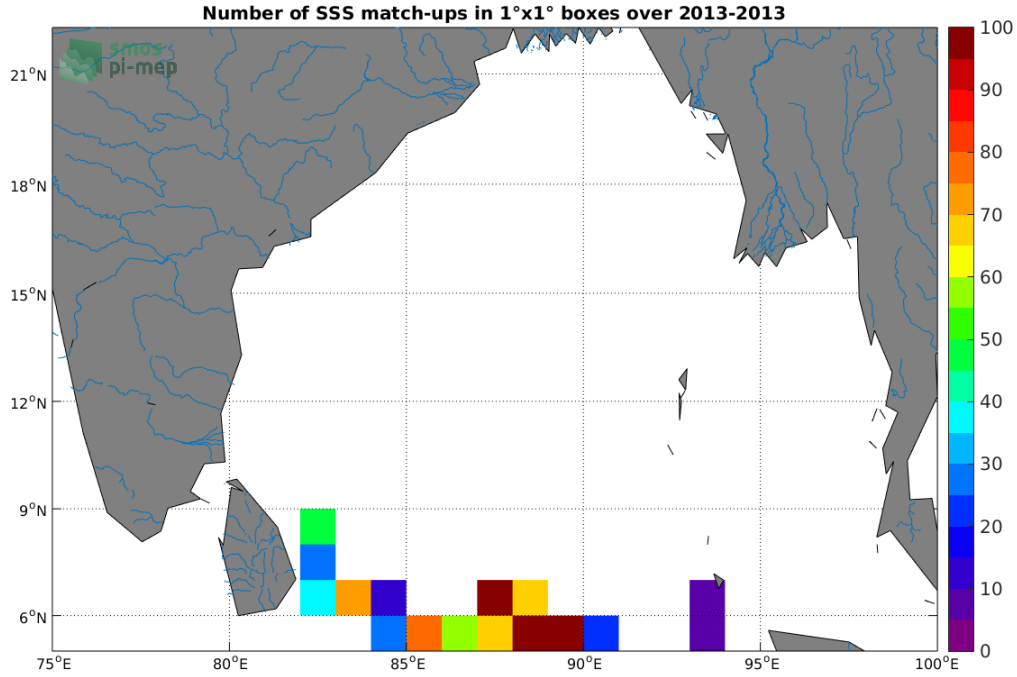
Figure 3: Number of SSS match-ups between Surface drifters SSS and the SMOS-L3-ICDC-V3-MONTHLY-0.5DEG SSS product for the Ganga and Brahmaputra river plumes Pi-MEP region over 1^\circ \times 1^\circ boxes and for the full satellite product period.
