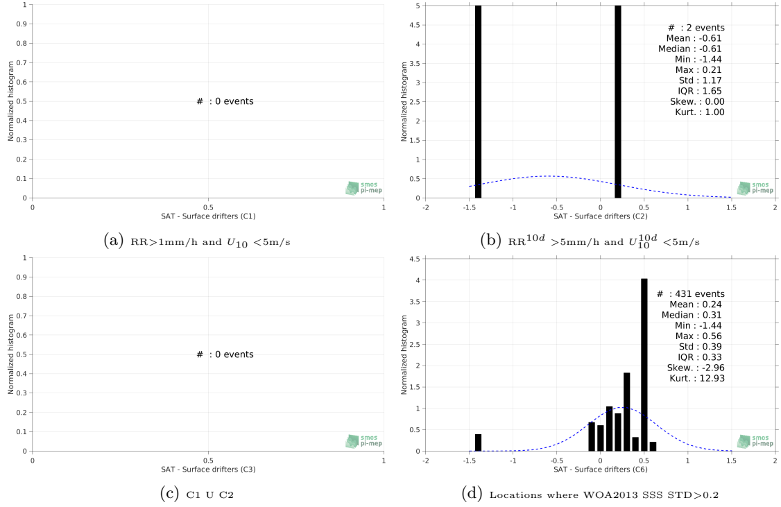
Figure 12: Normalized histogram of \Delta\text{SSS} (SMOS-L3-ICDC-V3-MONTHLY-0.5DEG - Surface drifters) for 6 different subdatasets corresponding to: RR > 1\text{mm/h} and U_{10} < 5\text{m/s} (a), RR^{10d} > 5\text{mm/h} and U_{10}^{10d} < 5\text{m/s} (b), C1 \cup C2 (c), Locations where WOA2013 SSS STD > 0.2 (d).
