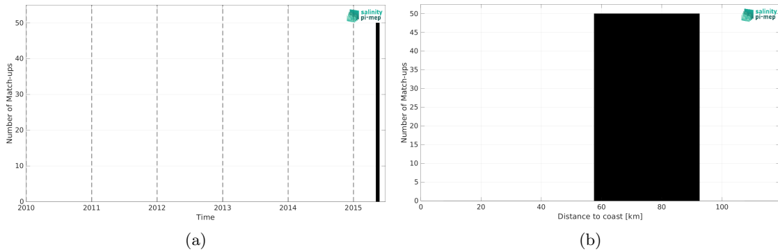
Figure 2: Number of match-ups between TSG (SAMOS) and SMOS SSS L2Q v331 - With FLAG (CMEMS-CATDS-CPDC) SSS as a function of time (a) and as function of the distance to coast (b) over the Ganga and Brahmaputra river plumes Pi-MEP region and for the full satellite product period.
