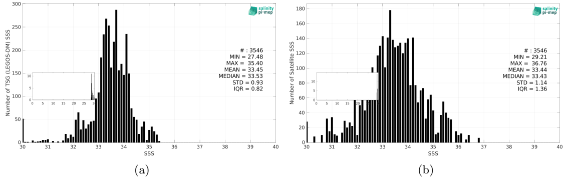
Figure 3: Histograms of SSS from TSG (LEGOS-DM) (a) and SMOS SSS L2Q v331 - With FLAG (CMEMS-CATDS-CPDC) (b) considering all match-up pairs per bins of 0.1 over the Ganga and Brahmaputra river plumes Pi-MEP region and for the full satellite product period.
