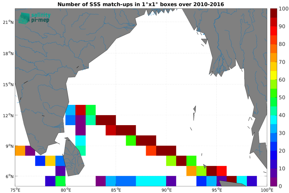
Figure 5: Number of SSS match-ups between TSG (LEGOS-DM) SSS and the SMOS SSS L2Q v331 - With FLAG (CMEMS-CATDS-CPDC) SSS product for the Ganga and Brahmaputra river plumes Pi-MEP region over 1^\circ \times 1^\circ boxes and for the full satellite product period.
