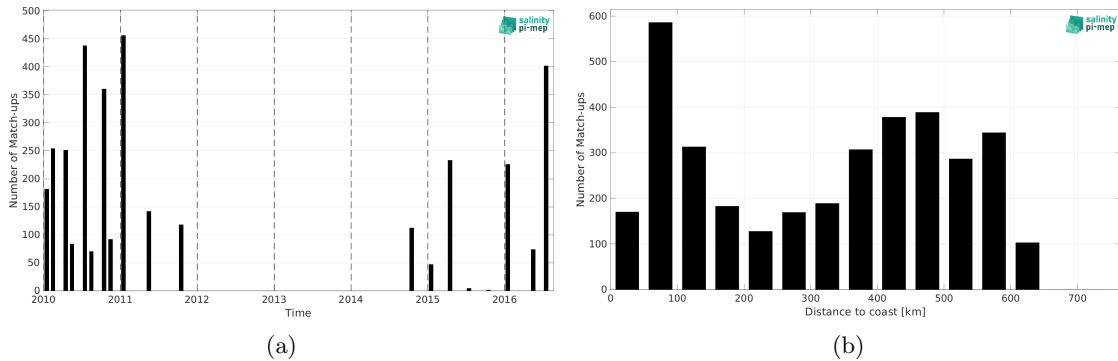
Figure 2: Number of match-ups between TSG (LEGOS-DM) and SMOS SSS L2Q v331 - With FLAG (CMEMS-CATDS-CPDC) SSS as a function of time (a) and as function of the distance to coast (b) over the Ganga and Brahmaputra river plumes Pi-MEP region and for the full satellite product period.
