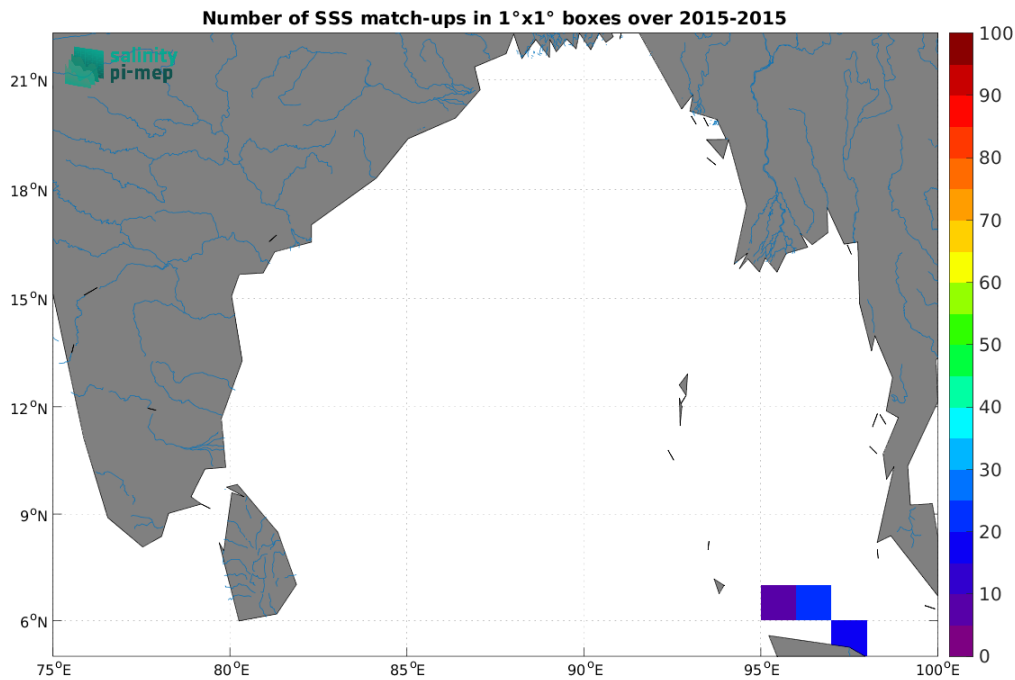
Figure 5: Number of SSS match-ups between TSG (SAMOS) SSS and the SMOS SSS L2Q v331 - No FLAG (CMEMS-CATDS-CPDC) SSS product for the Ganga and Brahmaputra river plumes Pi-MEP region over 1^{\circ} \times 1^{\circ} boxes and for the full satellite product period.
