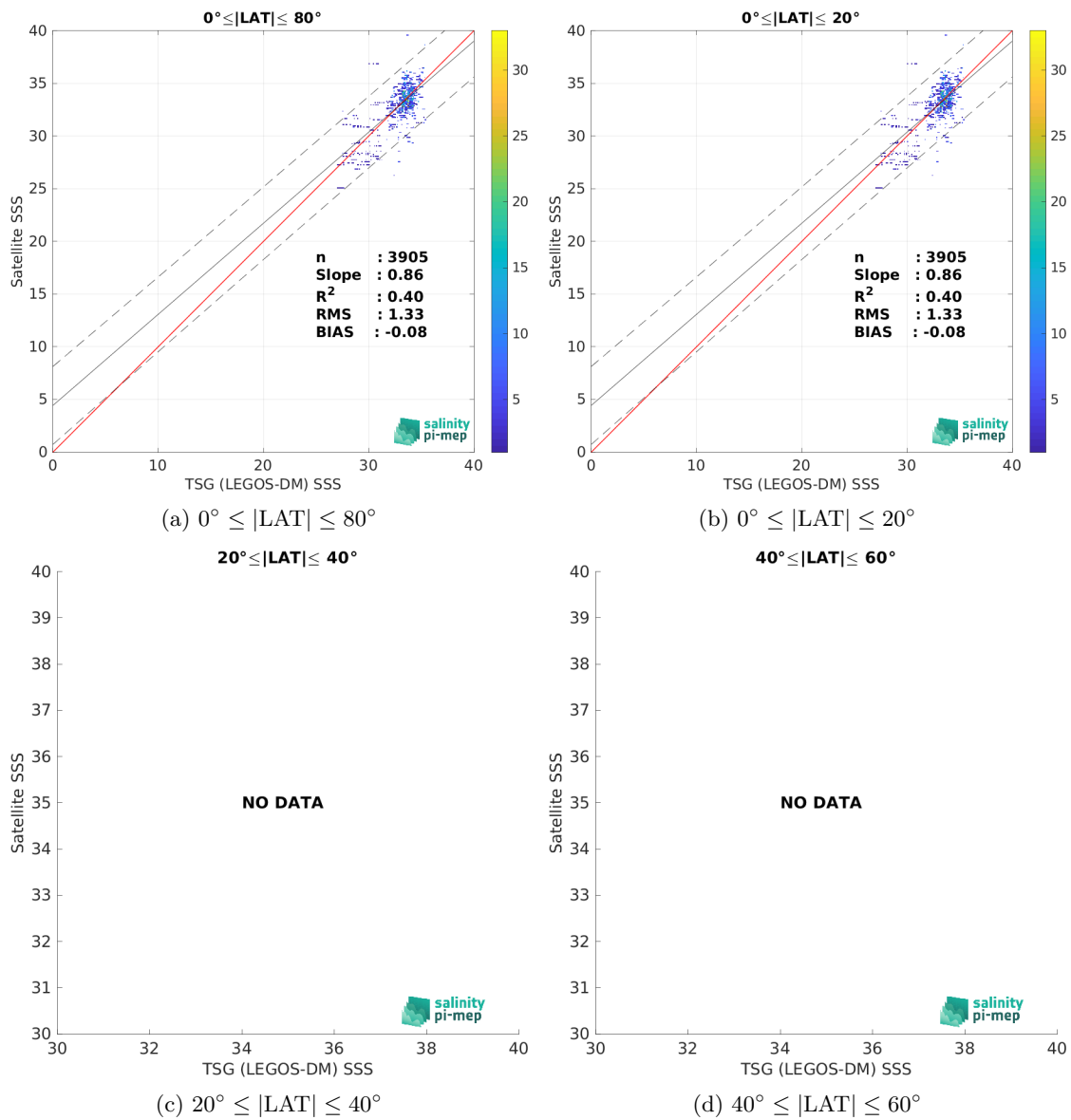
Figure 10: Contour maps of the concentration of SMOS SSS L2Q v331 - No FLAG (CMEMS-CATDS-CPDC) SSS (y-axis) versus TSG (LEGOS-DM) SSS (x-axis) at match-up pairs for different latitude bands. For each plot, the red line shows x=y . The black thin and dashed lines indicate a linear fit through the data cloud and the \pm 95\% confidence levels, respectively. The number match-up pairs n , the slope and R^2 coefficient of the linear fit, the root mean square (RMS) and the mean bias between satellite and in situ data are indicated for each latitude band in each plots.
