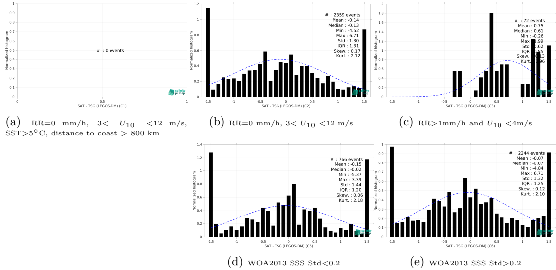
Figure 15: Normalized histogram of \Delta SSS (SMOS SSS L2Q v331 - No FLAG (CMEMS-CATDS-CPDC) - TSG (LEGOS-DM)) for 5 different subdatasets corresponding to: RR=0 mm/h, 3 < U_{10} < 12 m/s, SST>5°C, distance to coast > 800 km (a), RR=0 mm/h, 3 < U_{10} < 12 m/s (b), RR>1mm/h and U_{10} < 4 m/s (c), WOA2013 SSS Std<0.2 (d), WOA2013 SSS Std>0.2 (e).
