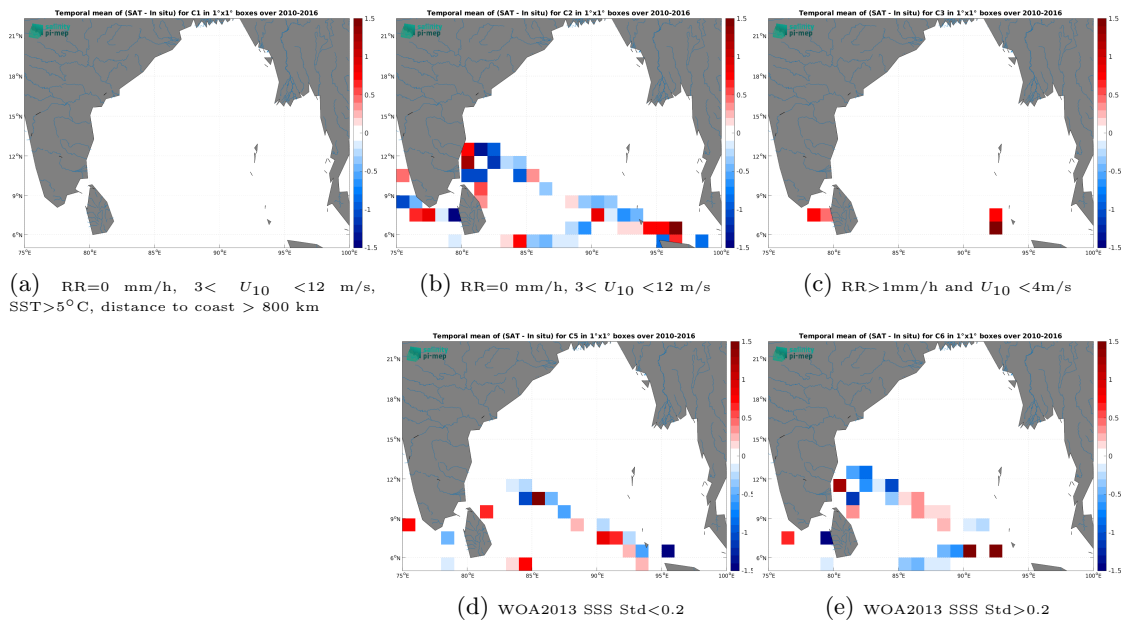
Figure 14: Temporal mean gridded over spatial boxes of size 1^\circ \times 1^\circ of \Delta SSS (SMOS SSS L2Q v331 - No FLAG (CMEMS-CATDS-CPDC) - TSG (LEGOS-DM)) for 5 different subdatasets corresponding to:RR=0 mm/h, 3 < U_{10} < 12 m/s, SST>5°C, distance to coast > 800 km (a), RR=0 mm/h, 3 < U_{10} < 12 m/s (b), RR>1mm/h and U_{10} < 4 m/s (c), WOA2013 SSS Std<0.2 (d), WOA2013 SSS Std>0.2 (e).
