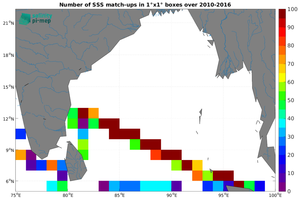
Figure 5: Number of SSS match-ups between TSG (LEGOS-DM) SSS and the SMOS SSS L2Q v331 - No FLAG (CMEMS-CATDS-CPDC) SSS product for the Ganga and Brahmaputra river plumes Pi-MEP region over 1^\circ \times 1^\circ boxes and for the full satellite product period.
