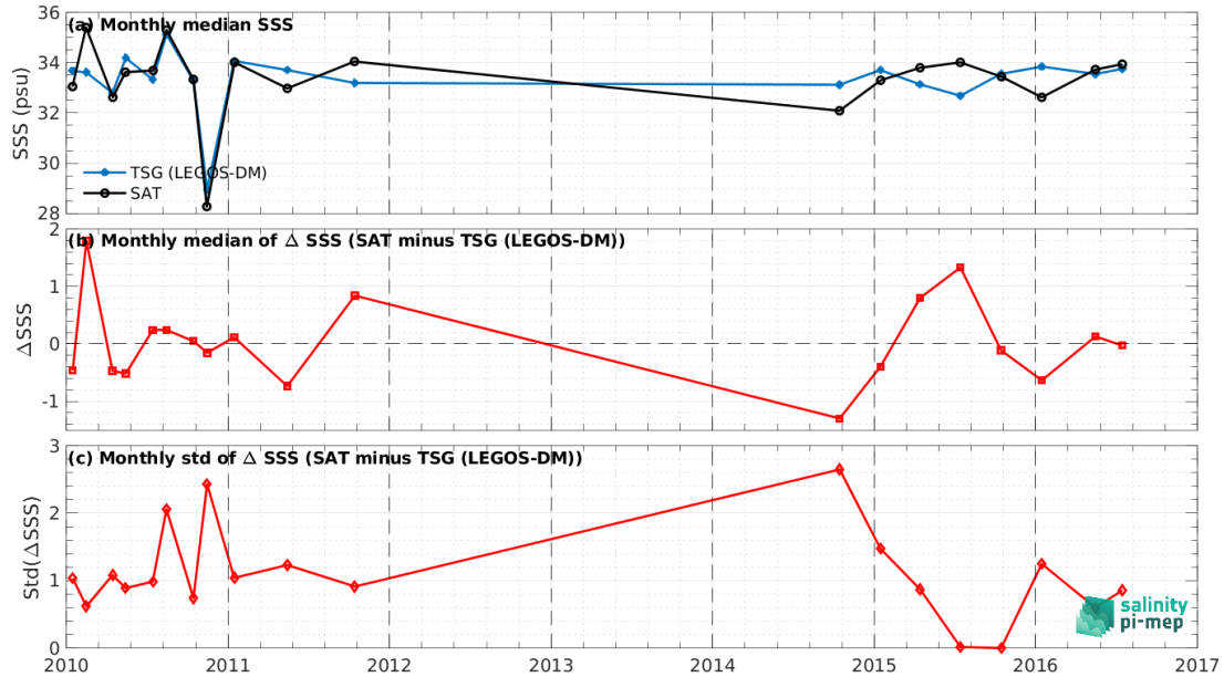
Figure 8: Time series of the monthly median SSS (top), median of \Delta SSS (Satellite - TSG (LEGOS-DM)) and Std of \Delta SSS (Satellite - TSG (LEGOS-DM)) over the Ganga and Brahmaputra river plumes Pi-MEP region considering all match-ups collected by the Pi-MEP.
