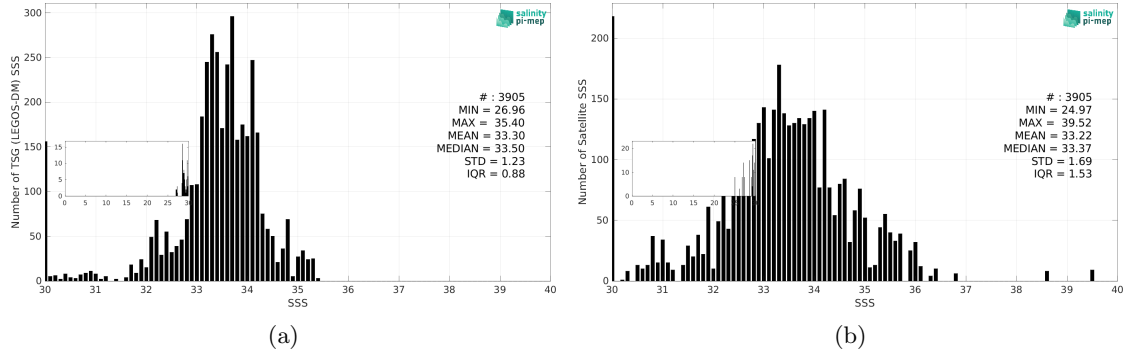
Figure 3: Histograms of SSS from TSG (LEGOS-DM) (a) and SMOS SSS L2Q v331 - No FLAG (CMEMS-CATDS-CPDC) (b) considering all match-up pairs per bins of 0.1 over the Ganga and Brahmaputra river plumes Pi-MEP region and for the full satellite product period.
