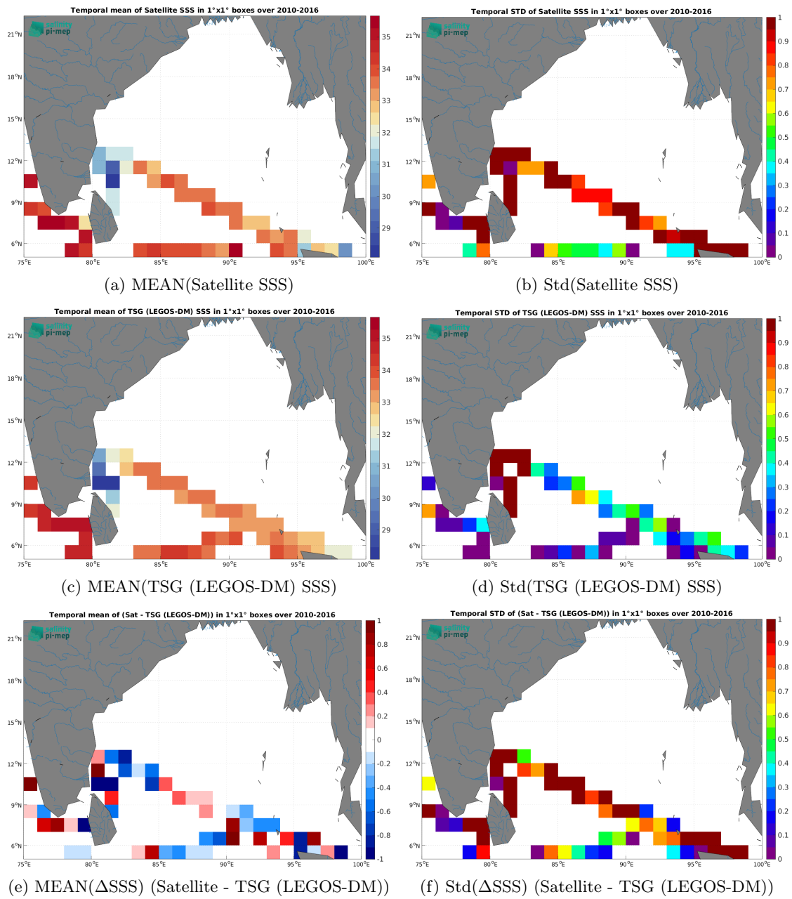
Figure 7: Temporal mean (left) and Std (right) of SSS from SMOS SSS L2Q v331 - No FLAG (CMEMS-CATDS-CPDC) (top), TSG (LEGOS-DM) (middle), and of \Delta SSS (Satellite - TSG (LEGOS-DM)). Only match-up pairs are used to generate these maps.
