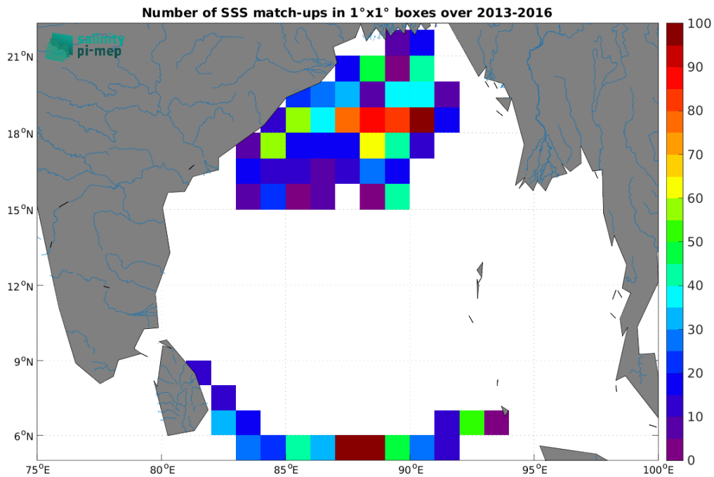
Figure 4: Number of SSS match-ups between Surface drifters SSS and the SMOS SSS L2Q v331 - No FLAG (CMEMS-CATDS-CPDC) SSS product for the Ganga and Brahmaputra river plumes Pi-MEP region over 1^\circ \times 1^\circ boxes and for the full satellite product period.
