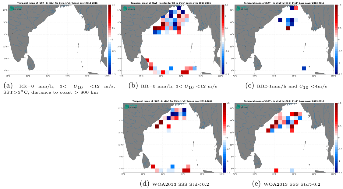
Figure 13: Temporal mean gridded over spatial boxes of size 1^\circ \times 1^\circ of \Delta SSS (SMOS SSS L2Q v331 - No FLAG (CMEMS-CATDS-CPDC) - Surface drifters) for 5 different subdatasets corresponding to:RR=0 mm/h, 3 < U_{10} < 12 m/s, SST >5^\circ C, distance to coast > 800 km (a), RR=0 mm/h, 3 < U_{10} < 12 m/s (b), RR >1 mm/h and U_{10} < 4 m/s (c), WOA2013 SSS Std <0.2 (d), WOA2013 SSS Std >0.2 (e).
