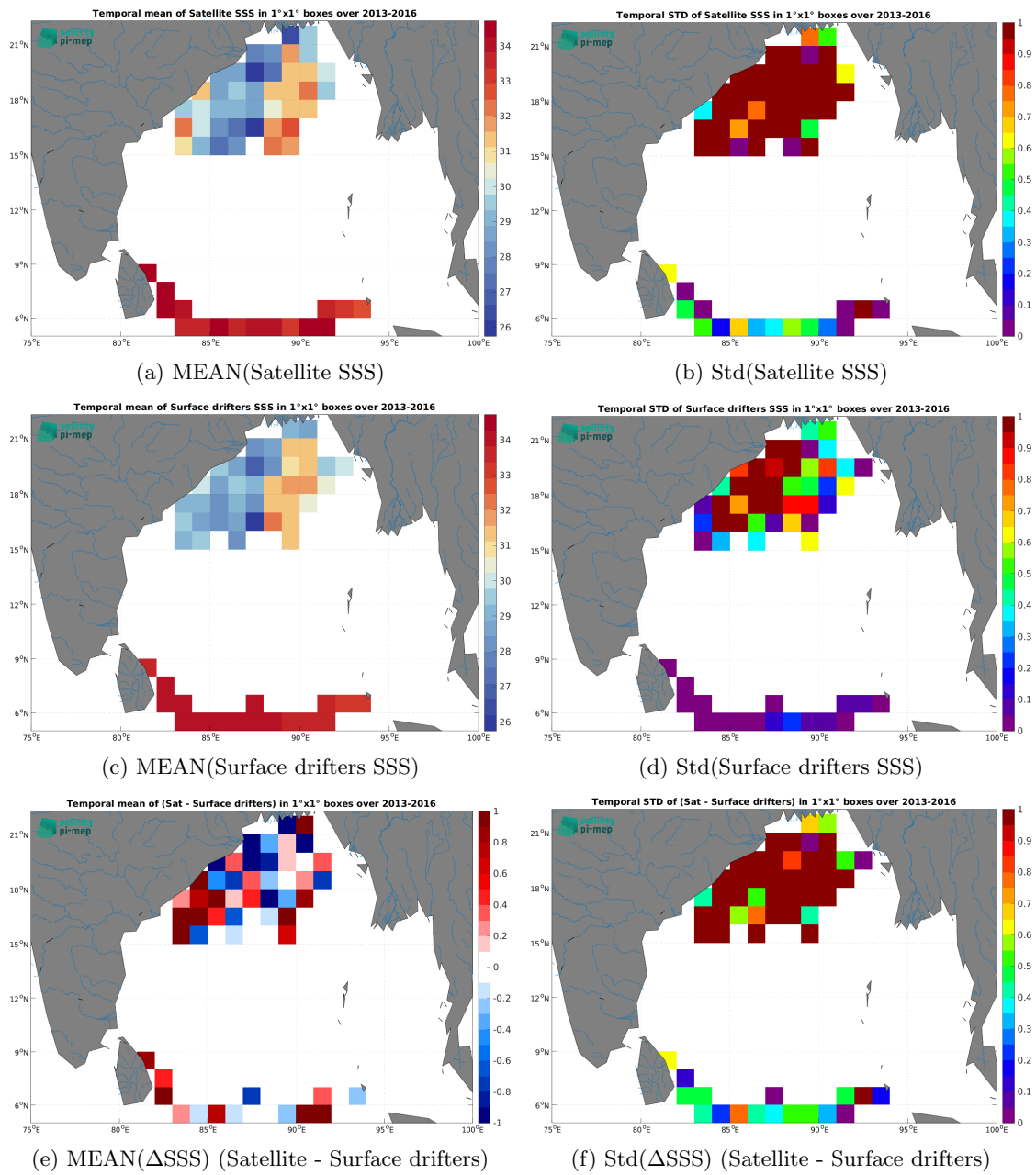
Figure 6: Temporal mean (left) and Std (right) of SSS from SMOS SSS L2Q v331 - No FLAG (CMEMS-CATDS-CPDC) (top), Surface drifters (middle), and of \Delta SSS (Satellite - Surface drifters). Only match-up pairs are used to generate these maps.
