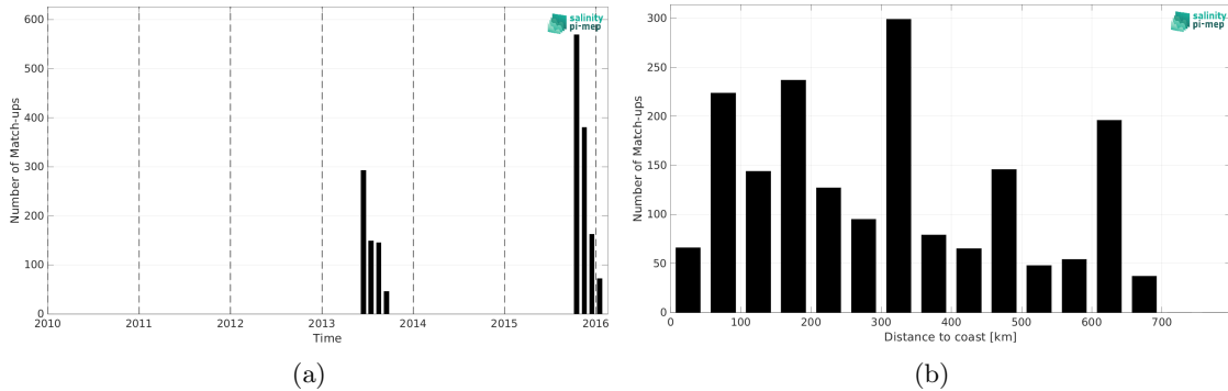
Figure 2: Number of match-ups between Surface drifters and SMOS SSS L2Q v331 - No FLAG (CMEMS-CATDS-CPDC) SSS as a function of time (a) and as function of the distance to coast (b) over the Ganga and Brahmaputra river plumes Pi-MEP region and for the full satellite product period.
