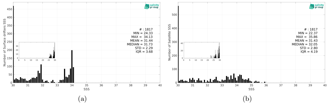
Figure 3: Histograms of SSS from Surface drifters (a) and SMOS SSS L2Q v331 - No FLAG (CMEMS-CATDS-CPDC) (b) considering all match-up pairs per bins of 0.1 over the Ganga and Brahmaputra river plumes Pi-MEP region and for the full satellite product period.
