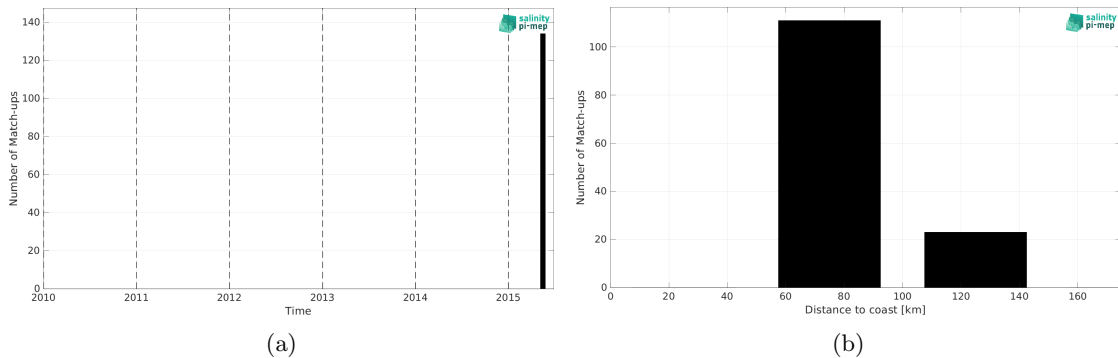
Figure 2: Number of match-ups between TSG (SAMOS) and SMOS SSS L3 v9 - 9 Days (CATDS-CEC-LOCEAN) SSS as a function of time (a) and as function of the distance to coast (b) over the Ganga and Brahmaputra river plumes Pi-MEP region and for the full satellite product period.
