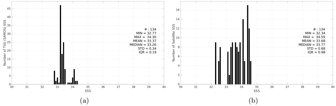
Figure 3: Histograms of SSS from TSG (SAMOS) (a) and SMOS SSS L3 v9 - 9 Days (CATDS-CEC-LOCEAN) (b) considering all match-up pairs per bins of 0.1 over the Ganga and Brahmaputra river plumes Pi-MEP region and for the full satellite product period.
