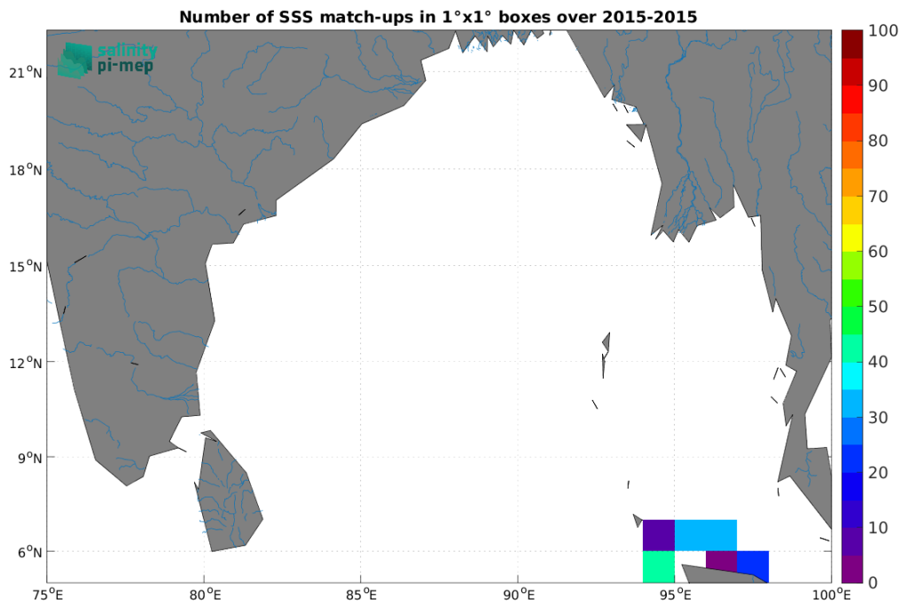
Figure 5: Number of SSS match-ups between TSG (SAMOS) SSS and the SMOS SSS L3 v9 - 9 Days (CATDS-CEC-LOCEAN) SSS product for the Ganga and Brahmaputra river plumes Pi-MEP region over 1^\circ \times 1^\circ boxes and for the full satellite product period.
