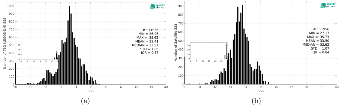
Figure 2: Histograms of SSS from TSG (LEGOS-DM) (a) and SMOS SSS L3 v9 - 9 Days (CATDS-CEC-LOCEAN) (b) considering all match-up pairs per bins of 0.1 over the Ganga and Brahmaputra river plumes Pi-MEP region and for the full satellite product period.
