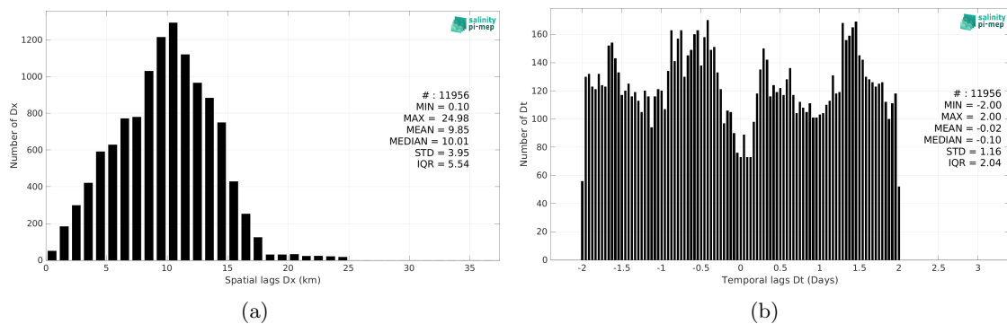
Figure 5: Histograms of the spatial (a) and temporal (b) lags between the location/time of the TSG (LEGOS-DM) measurement and the date of the corresponding SMOS SSS L3 v9 - 9 Days (CATDS-CEC-LOCEAN) SSS pixel.
