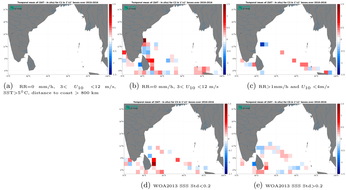
Figure 12: Temporal mean gridded over spatial boxes of size 1^{\circ}\times 1^{\circ} of \Delta\text{SSS} (SMOS SSS L3 v9 - 9 Days (CATDS-CEC-LOCEAN) - TSG (LEGOS-DM)) for 5 different subdatasets corresponding to:RR=0 mm/h, 3 < U_{10} < 12 m/s, SST >5^{\circ}\text{C} , distance to coast > 800 km (a), RR=0 mm/h, 3 < U_{10} < 12 m/s (b), RR >1 mm/h and U_{10} < 4 m/s (c), WOA2013 SSS Std <0.2 (d), WOA2013 SSS Std >0.2 (e).
