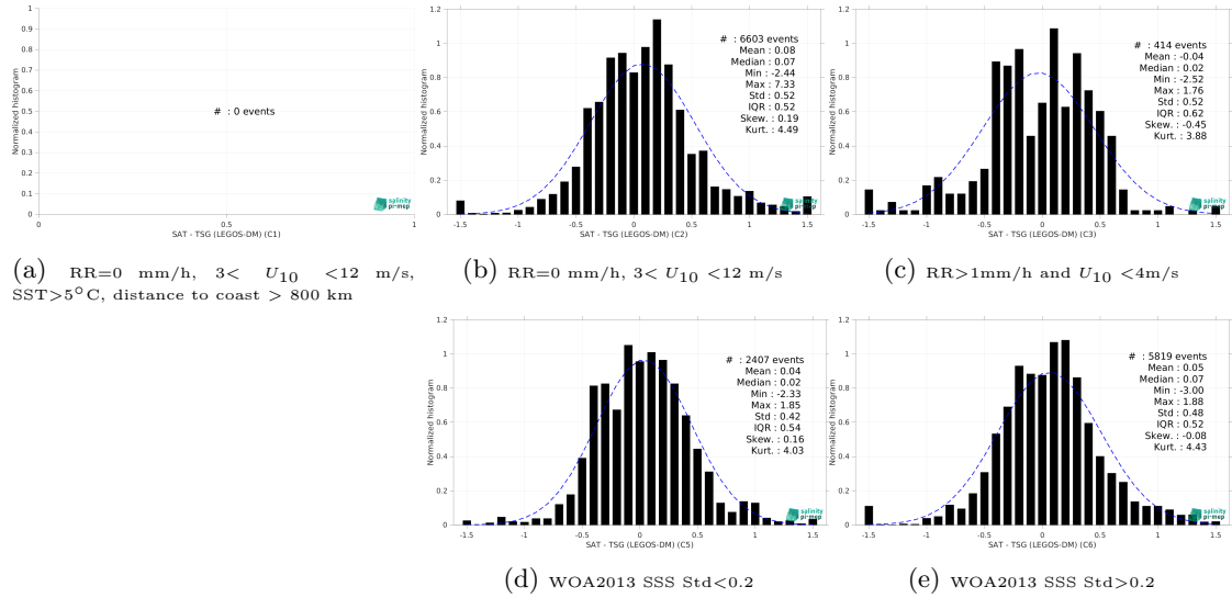
Figure 13: Normalized histogram of \Delta SSS (SMOS SSS L3 v9 - 9 Days (CATDS-CEC-LOCEAN) - TSG (LEGOS-DM)) for 5 different subdatasets corresponding to: RR=0 mm/h, 3 < U_{10} < 12 m/s, SST > 5°C, distance to coast > 800 km (a), RR=0 mm/h, 3 < U_{10} < 12 m/s (b), RR > 1mm/h and U_{10} < 4 m/s (c), WOA2013 SSS Std < 0.2 (d), WOA2013 SSS Std > 0.2 (e).
