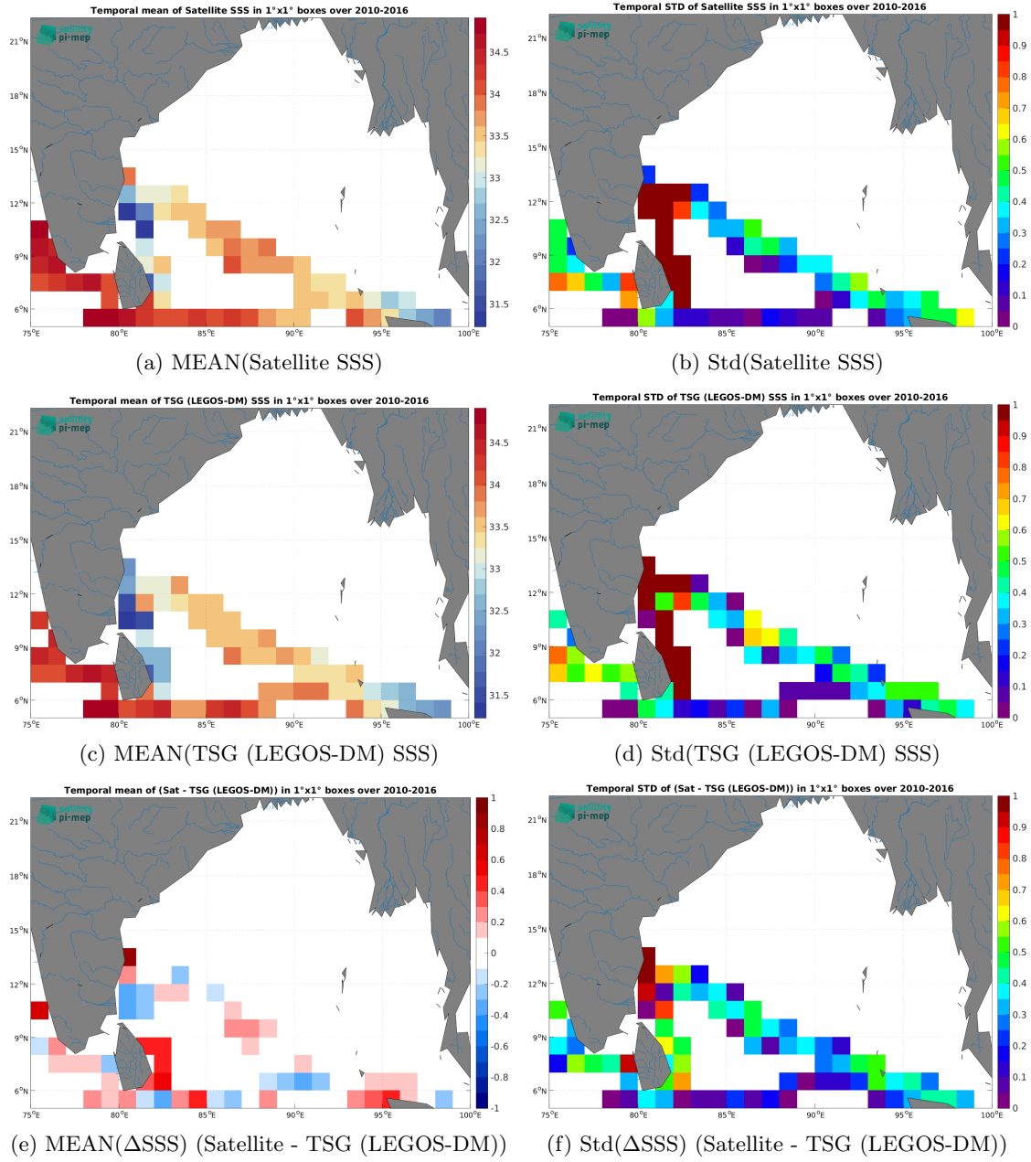
Figure 6: Temporal mean (left) and Std (right) of SSS from SMOS SSS L3 v9 - 9 Days (CATDS-CEC-LOCEAN) (top), TSG (LEGOS-DM) (middle), and of \Delta SSS (Satellite - TSG (LEGOS-DM)). Only match-up pairs are used to generate these maps.
