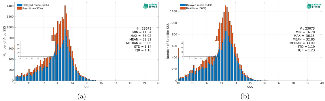
Figure 3: Histograms of SSS from Argo (a) and SMOS SSS L3 v9 - 9 Days (CATDS-CEC-LOCEAN) (b) considering all match-up pairs per bins of 0.1 over the Ganga and Brahmaputra river plumes Pi-MEP region and for the full satellite product period.
