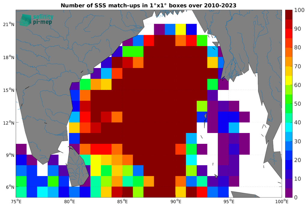
Figure 5: Number of SSS match-ups between Argo SSS and the SMOS SSS L3 v9 - 9 Days (CATDS-CEC-LOCEAN) SSS product for the Ganga and Brahmaputra river plumes Pi-MEP region over 1^\circ \times 1^\circ boxes and for the full satellite product period.
