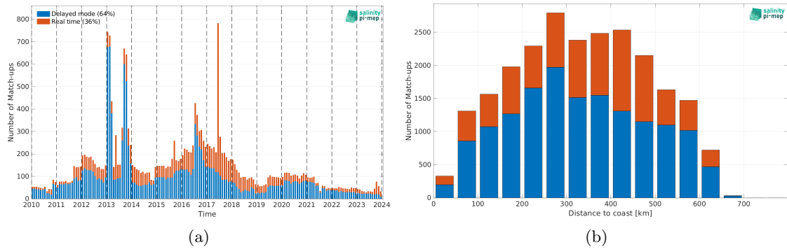
Figure 2: Number of match-ups between Argo and SMOS SSS L3 v9 - 9 Days (CATDS-CEC-LOCEAN) SSS as a function of time (a) and as function of the distance to coast (b) over the Ganga and Brahmaputra river plumes Pi-MEP region and for the full satellite product period.
