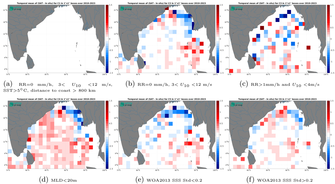
Figure 14: Temporal mean gridded over spatial boxes of size 1^\circ \times 1^\circ of \Delta SSS (SMOS SSS L3 v9 - 9 Days (CATDS-CEC-LOCEAN) - Argo) for 6 different subdatasets corresponding to:RR=0 mm/h, 3 < U_{10} < 12 m/s, SST >5^\circ C, distance to coast > 800 km (a), RR=0 mm/h, 3 < U_{10} < 12 m/s (b), RR >1 mm/h and U_{10} < 4 m/s (c),MLD <20 m (d),WOA2013 SSS Std <0.2 (e),WOA2013 SSS Std >0.2 (f).
