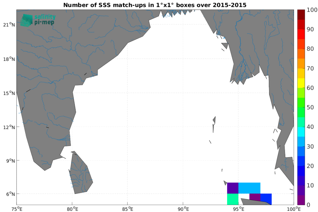
Figure 5: Number of SSS match-ups between TSG (SAMOS) SSS and the SMOS SSS L3 v9 - 18 Days (CATDS-CEC-LOCEAN) SSS product for the Ganga and Brahmaputra river plumes Pi-MEP region over 1^\circ \times 1^\circ boxes and for the full satellite product period.
