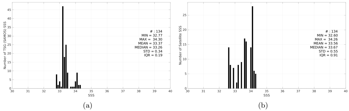
Figure 3: Histograms of SSS from TSG (SAMOS) (a) and SMOS SSS L3 v9 - 18 Days (CATDS-CEC-LOCEAN) (b) considering all match-up pairs per bins of 0.1 over the Ganga and Brahmaputra river plumes Pi-MEP region and for the full satellite product period.
