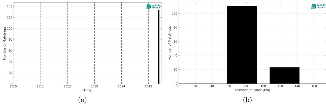
Figure 2: Number of match-ups between TSG (SAMOS) and SMOS SSS L3 v9 - 18 Days (CATDS-CEC-LOCEAN) SSS as a function of time (a) and as function of the distance to coast (b) over the Ganga and Brahmaputra river plumes Pi-MEP region and for the full satellite product period.
