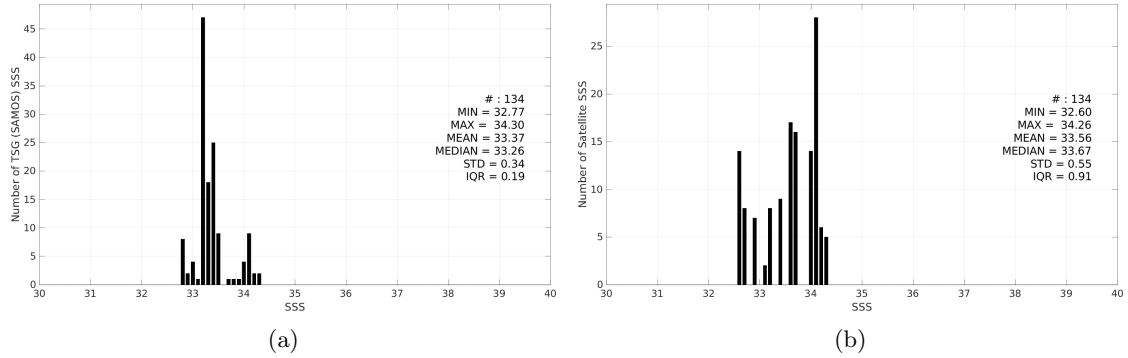
Figure 2: Histograms of SSS from TSG (SAMOS) (a) and SMOS SSS L3 v9 - 18 Days (CATDS-CEC-LOCEAN) (b) considering all match-up pairs per bins of 0.1 over the Ganga and Brahmaputra river plumes Pi-MEP region and for the full satellite product period.
