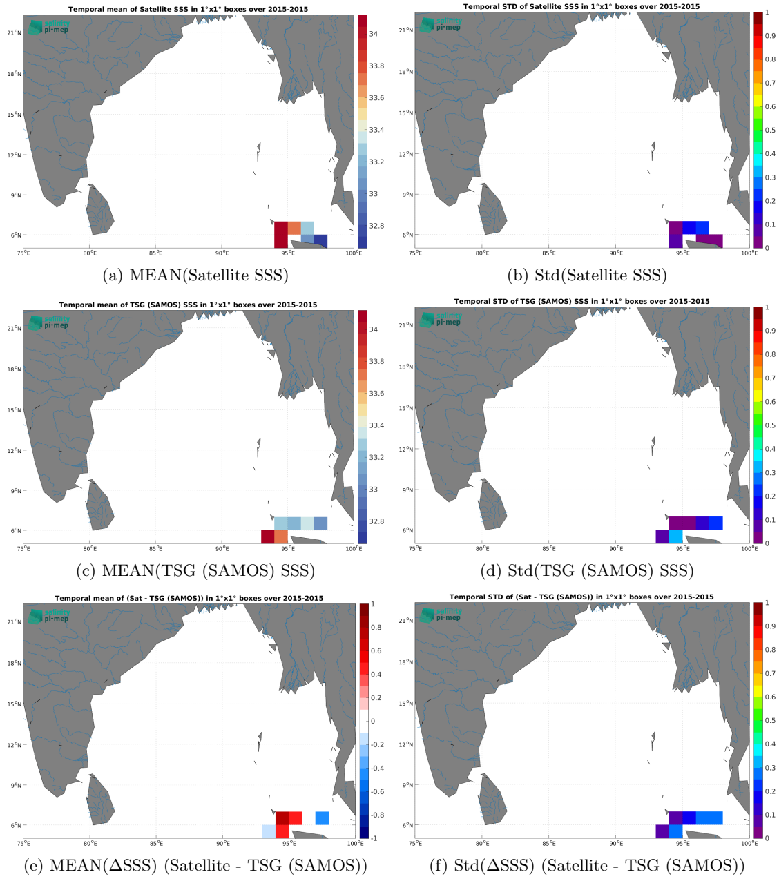
Figure 6: Temporal mean (left) and Std (right) of SSS from SMOS SSS L3 v9 - 18 Days (CATDS-CEC-LOCEAN) (top), TSG (SAMOS) (middle), and of \Delta SSS (Satellite - TSG (SAMOS)). Only match-up pairs are used to generate these maps.
