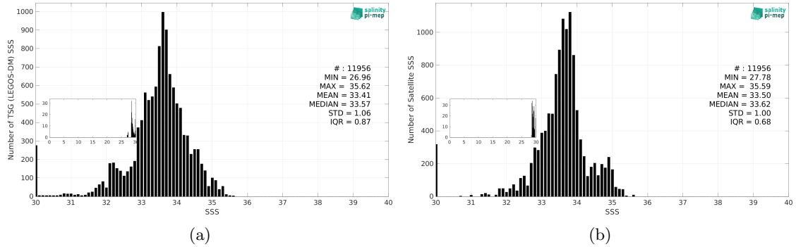
Figure 3: Histograms of SSS from TSG (LEGOS-DM) (a) and SMOS SSS L3 v9 - 18 Days (CATDS-CEC-LOCEAN) (b) considering all match-up pairs per bins of 0.1 over the Ganga and Brahmaputra river plumes Pi-MEP region and for the full satellite product period.
