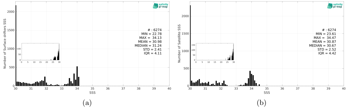
Figure 3: Histograms of SSS from Surface drifters (a) and SMOS SSS L3 v9 - 18 Days (CATDS-CEC-LOCEAN) (b) considering all match-up pairs per bins of 0.1 over the Ganga and Brahmaputra river plumes Pi-MEP region and for the full satellite product period.
