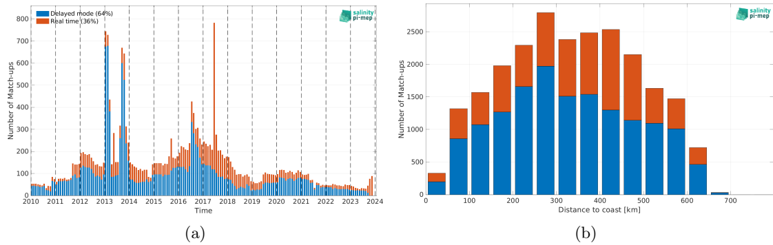
Figure 2: Number of match-ups between Argo and SMOS SSS L3 v9 - 18 Days (CATDS-CEC-LOCEAN) SSS as a function of time (a) and as function of the distance to coast (b) over the Ganga and Brahmaputra river plumes Pi-MEP region and for the full satellite product period.
