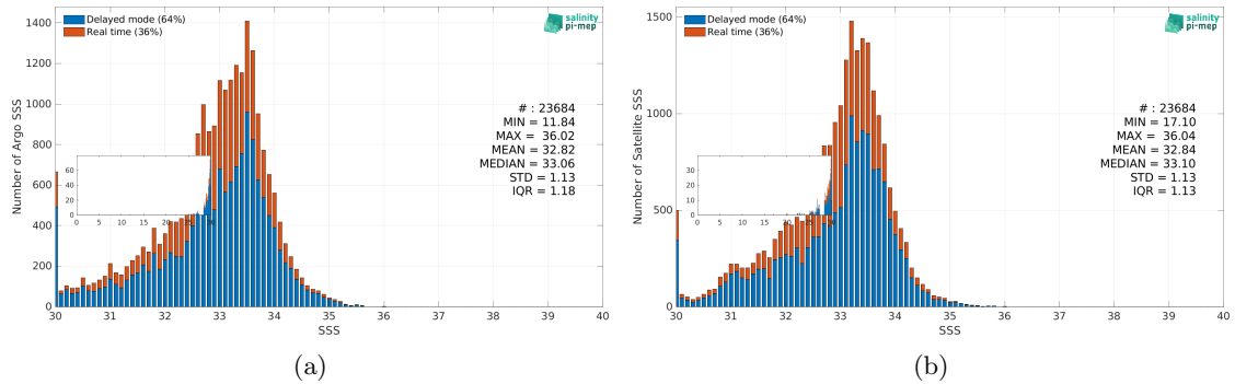
Figure 3: Histograms of SSS from Argo (a) and SMOS SSS L3 v9 - 18 Days (CATDS-CEC-LOCEAN) (b) considering all match-up pairs per bins of 0.1 over the Ganga and Brahmaputra river plumes Pi-MEP region and for the full satellite product period.
