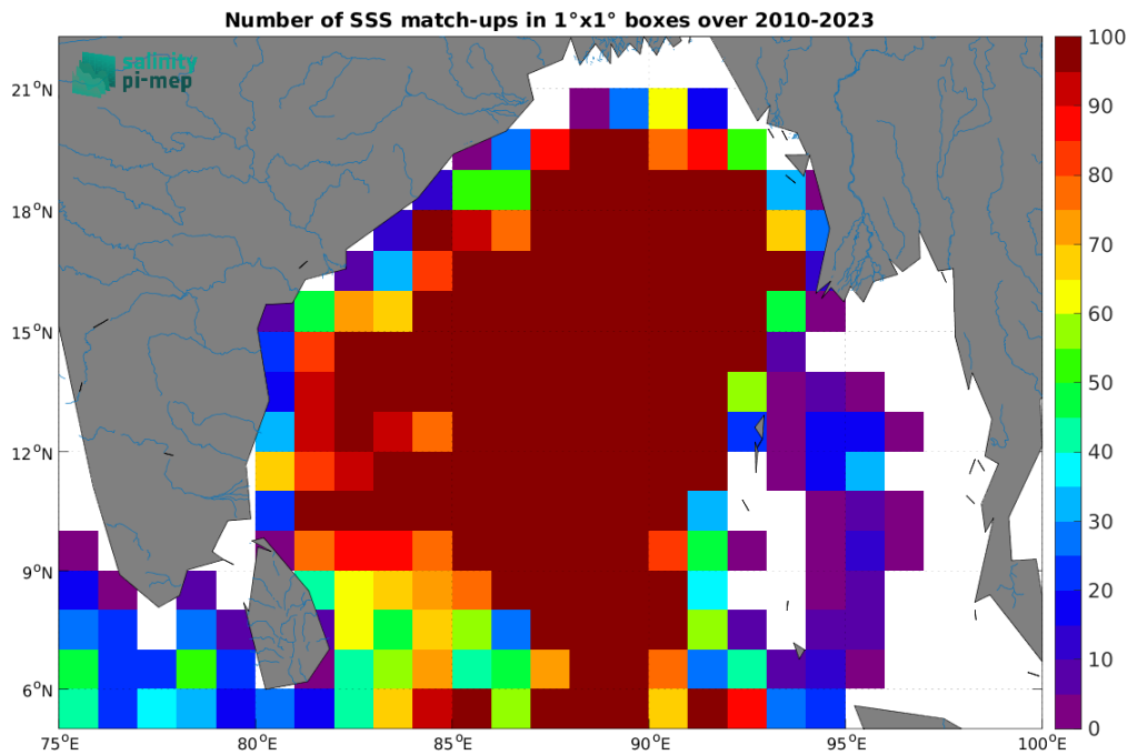
Figure 5: Number of SSS match-ups between Argo SSS and the SMOS SSS L3 v9 - 18 Days (CATDS-CEC-LOCEAN) SSS product for the Ganga and Brahmaputra river plumes Pi-MEP region over 1^\circ \times 1^\circ boxes and for the full satellite product period.
