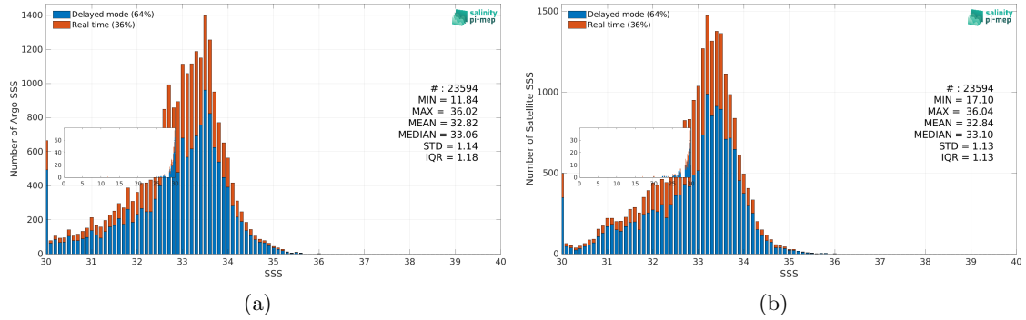
Figure 2: Histograms of SSS from Argo (a) and SMOS SSS L3 v9 - 18 Days (CATDS-CEC-LOCEAN) (b) considering all match-up pairs per bins of 0.1 over the Ganga and Brahmaputra river plumes Pi-MEP region and for the full satellite product period.
