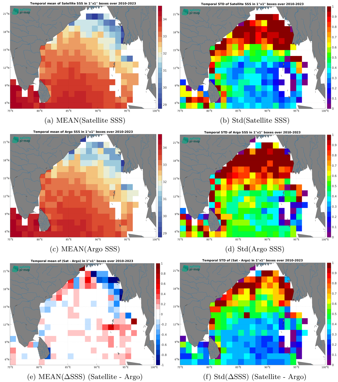
Figure 6: Temporal mean (left) and Std (right) of SSS from SMOS SSS L3 v9 - 18 Days (CATDS-CEC-LOCEAN) (top), Argo (middle), and of \Delta SSS (Satellite - Argo). Only match-up pairs are used to generate these maps.
