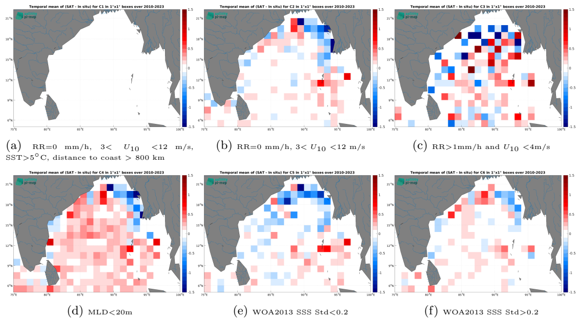
Figure 12: Temporal mean gridded over spatial boxes of size 1^\circ \times 1^\circ of \Delta SSS (SMOS SSS L3 v9 - 18 Days (CATDS-CEC-LOCEAN) - Argo) for 6 different subdatasets corresponding to:RR=0 mm/h, 3 < U_{10} < 12 m/s, SST >5^\circ C, distance to coast > 800 km (a), RR=0 mm/h, 3 < U_{10} < 12 m/s (b), RR >1 mm/h and U_{10} < 4 m/s (c),MLD <20 m (d),WOA2013 SSS Std <0.2 (e),WOA2013 SSS Std >0.2 (f).
