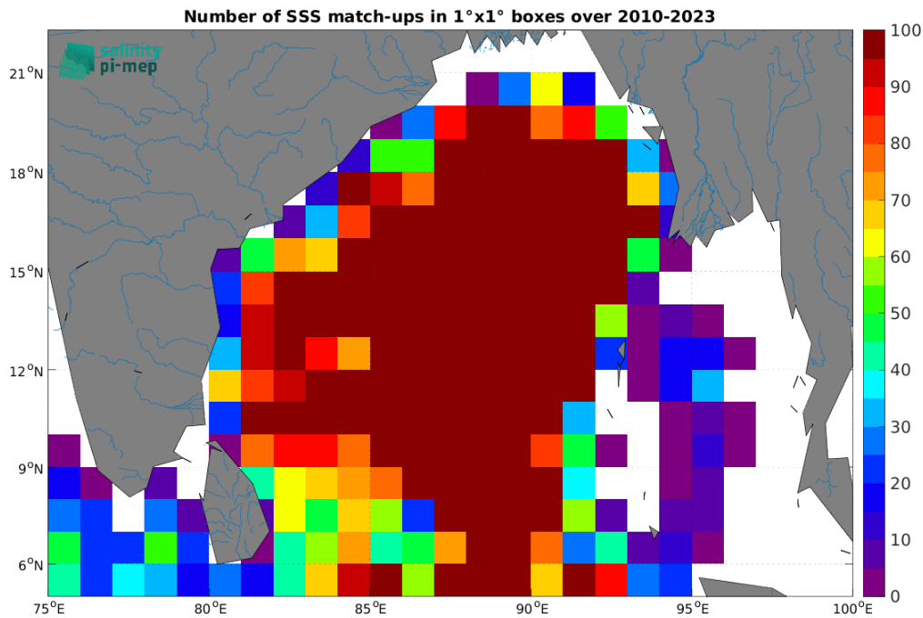
Figure 4: Number of SSS match-ups between Argo SSS and the SMOS SSS L3 v9 - 18 Days (CATDS-CEC-LOCEAN) SSS product for the Ganga and Brahmaputra river plumes Pi-MEP region over 1^\circ \times 1^\circ boxes and for the full satellite product period.
