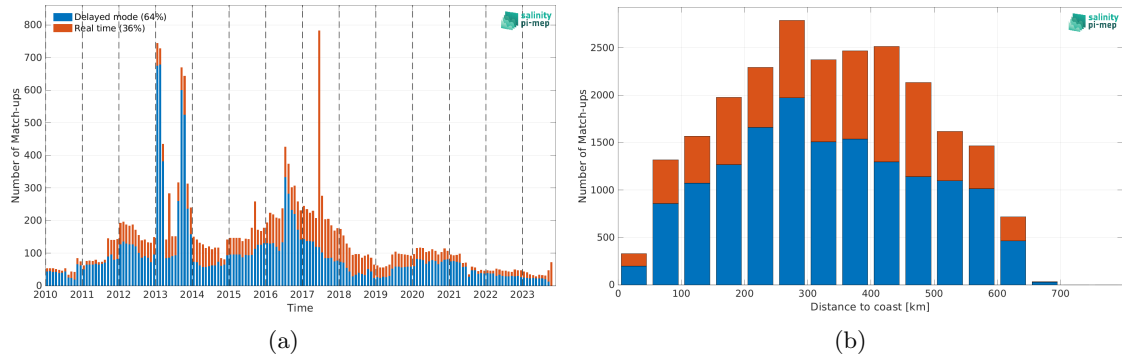
Figure 1: Number of match-ups between Argo and SMOS SSS L3 v9 - 18 Days (CATDS-CEC-LOCEAN) SSS as a function of time (a) and as function of the distance to coast (b) over the Ganga and Brahmaputra river plumes Pi-MEP region and for the full satellite product period.
