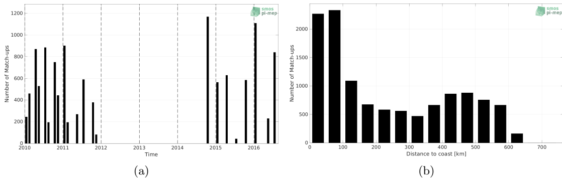
Figure 1: Number of match-ups between TSG (LEGOS-DM) and SMOS SSS L3 v8 - 9 Days (CATDS-CECOS-LOCEAN) SSS as a function of time (a) and as function of the distance to coast (b) over the Ganga and Brahmaputra river plumes Pi-MEP region and for the full satellite product period.
