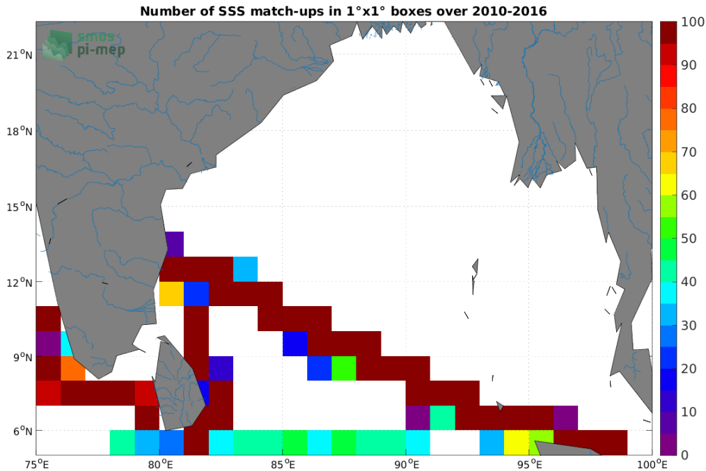
Figure 4: Number of SSS match-ups between TSG (LEGOS-DM) SSS and the SMOS SSS L3 v8 - 9 Days (CATDS-CECOS-LOCEAN) SSS product for the Ganga and Brahmaputra river plumes Pi-MEP region over 1^\circ \times 1^\circ boxes and for the full satellite product period.
