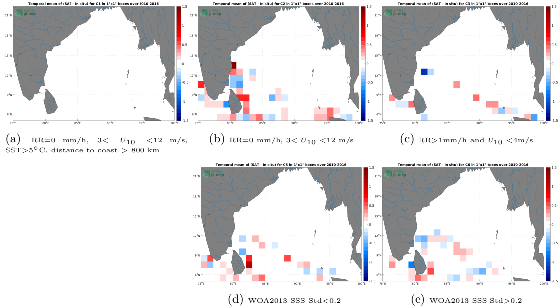
Figure 12: Temporal mean gridded over spatial boxes of size 1^{\circ}\times 1^{\circ} of \Delta\text{SSS} (SMOS SSS L3 v8 - 9 Days (CATDS-CECOS-LOCEAN) - TSG (LEGOS-DM)) for 5 different subdatasets corresponding to:RR=0 mm/h, 3 < U_{10} < 12 m/s, SST >5^{\circ}\text{C} , distance to coast > 800 km (a), RR=0 mm/h, 3 < U_{10} < 12 m/s (b), RR >1 mm/h and U_{10} < 4 m/s (c), WOA2013 SSS Std <0.2 (d), WOA2013 SSS Std >0.2 (e).
