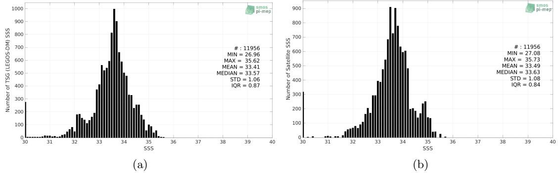
Figure 2: Histograms of SSS from TSG (LEGOS-DM) (a) and SMOS SSS L3 v8 - 9 Days (CATDS-CECOS-LOCEAN) (b) considering all match-up pairs per bins of 0.1 over the Ganga and Brahmaputra river plumes Pi-MEP region and for the full satellite product period.
