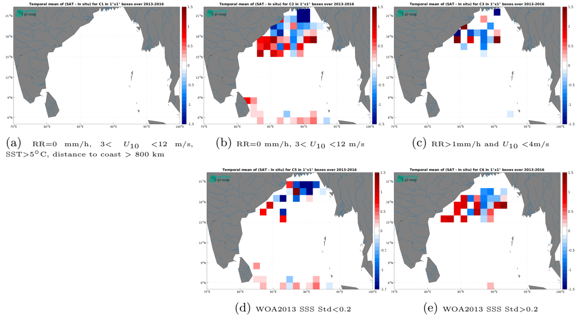
Figure 11: Temporal mean gridded over spatial boxes of size 1^{\circ}\times 1^{\circ} of \Delta\text{SSS} (SMOS SSS L3 v8 - 9 Days (CATDS-CEC-LOCEAN) - Surface drifters) for 5 different subdatasets corresponding to:RR=0 mm/h, 3 < U_{10} < 12 m/s, SST >5^{\circ}\text{C} , distance to coast > 800 km (a), RR=0 mm/h, 3 < U_{10} < 12 m/s (b), RR >1 mm/h and U_{10} < 4 m/s (c), WOA2013 SSS Std <0.2 (d), WOA2013 SSS Std >0.2 (e).
