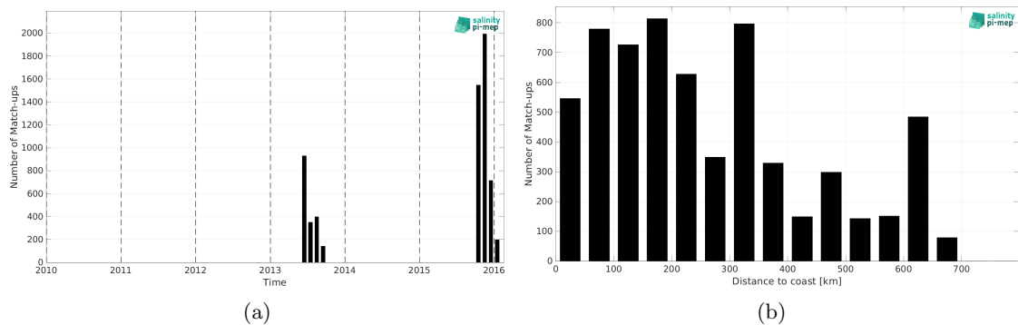
Figure 1: Number of match-ups between Surface drifters and SMOS SSS L3 v8 - 9 Days (CATDS-CEC-LOCEAN) SSS as a function of time (a) and as function of the distance to coast (b) over the Ganga and Brahmaputra river plumes Pi-MEP region and for the full satellite product period.
