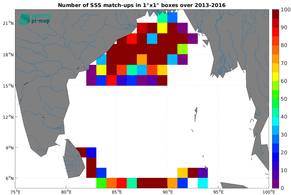
Figure 3: Number of SSS match-ups between Surface drifters SSS and the SMOS SSS L3 v8 - 9 Days (CATDS-CEC-LOCEAN) SSS product for the Ganga and Brahmaputra river plumes Pi-MEP region over 1^{\circ} \times 1^{\circ} boxes and for the full satellite product period.
