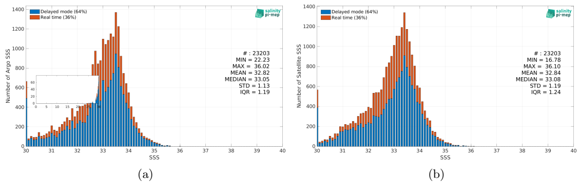
Figure 2: Histograms of SSS from Argo (a) and SMOS SSS L3 v8 - 9 Days (CATDS-CEC-LOCEAN) (b) considering all match-up pairs per bins of 0.1 over the Ganga and Brahmaputra river plumes Pi-MEP region and for the full satellite product period.
