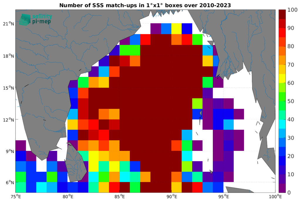
Figure 4: Number of SSS match-ups between Argo SSS and the SMOS SSS L3 v8 - 9 Days (CATDS-CEC-LOCEAN) SSS product for the Ganga and Brahmaputra river plumes Pi-MEP region over 1^\circ \times 1^\circ boxes and for the full satellite product period.
