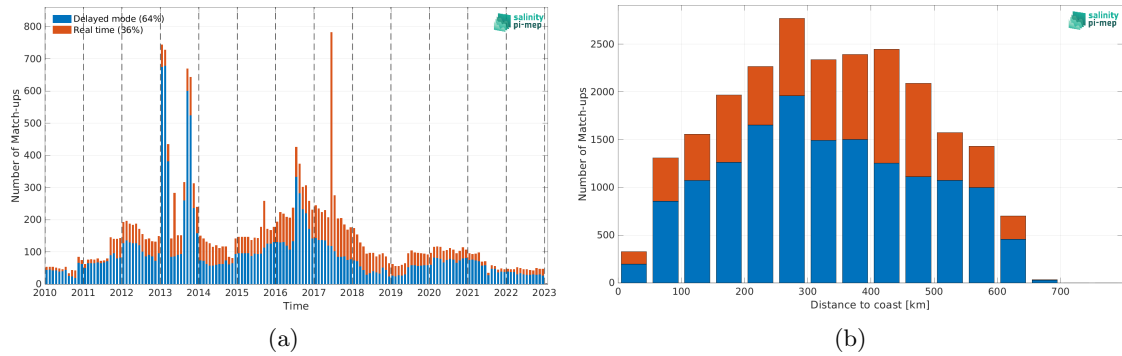
Figure 1: Number of match-ups between Argo and SMOS SSS L3 v8 - 9 Days (CATDS-CEC-LOCEAN) SSS as a function of time (a) and as function of the distance to coast (b) over the Ganga and Brahmaputra river plumes Pi-MEP region and for the full satellite product period.
