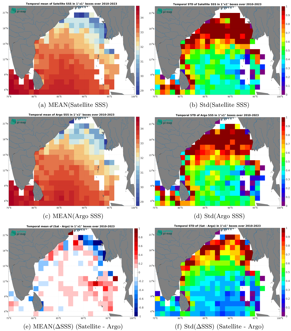
Figure 6: Temporal mean (left) and Std (right) of SSS from SMOS SSS L3 v8 - 9 Days (CATDS-CEC-LOCEAN) (top), Argo (middle), and of \Delta SSS (Satellite - Argo). Only match-up pairs are used to generate these maps.
