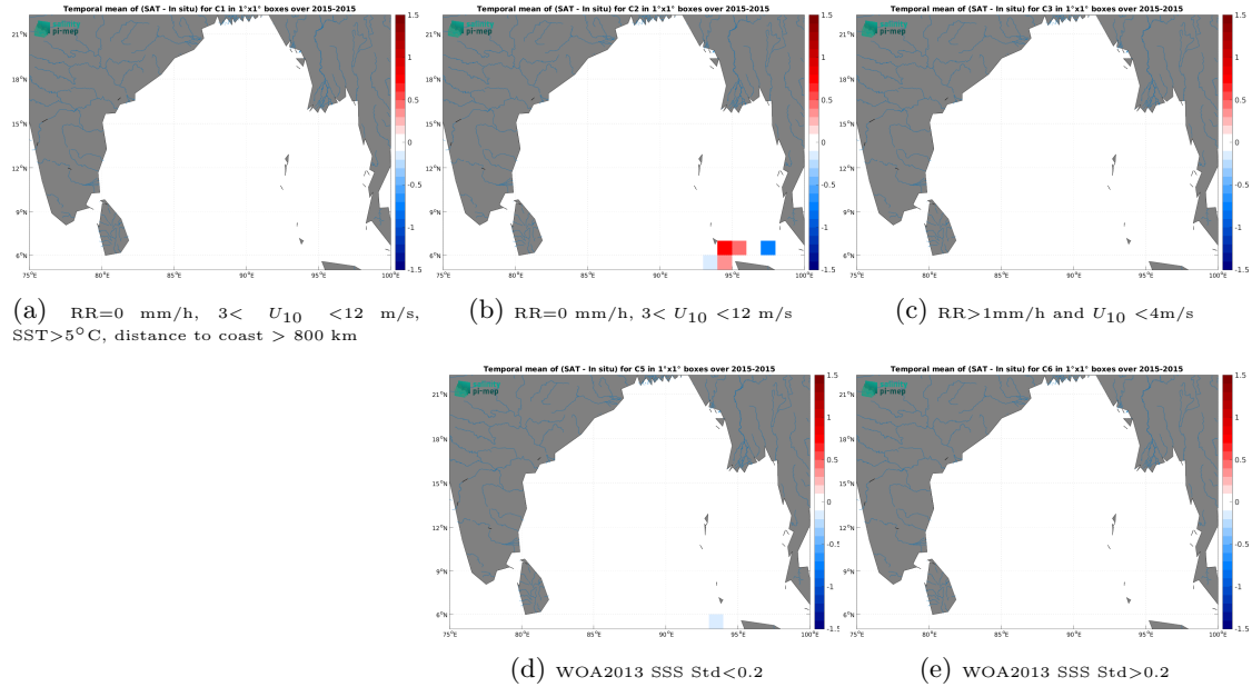
Figure 12: Temporal mean gridded over spatial boxes of size 1^{\circ}\times 1^{\circ} of \Delta\text{SSS} (SMOS SSS L3 v8 - 18 Days (CATDS-CEC-LOCEAN) - TSG (SAMOS)) for 5 different subdatasets corresponding to:RR=0 mm/h, 3 < U_{10} < 12 m/s, SST >5^{\circ}\text{C} , distance to coast > 800 km (a), RR=0 mm/h, 3 < U_{10} < 12 m/s (b), RR >1 mm/h and U_{10} < 4 m/s (c), WOA2013 SSS Std <0.2 (d), WOA2013 SSS Std >0.2 (e).
