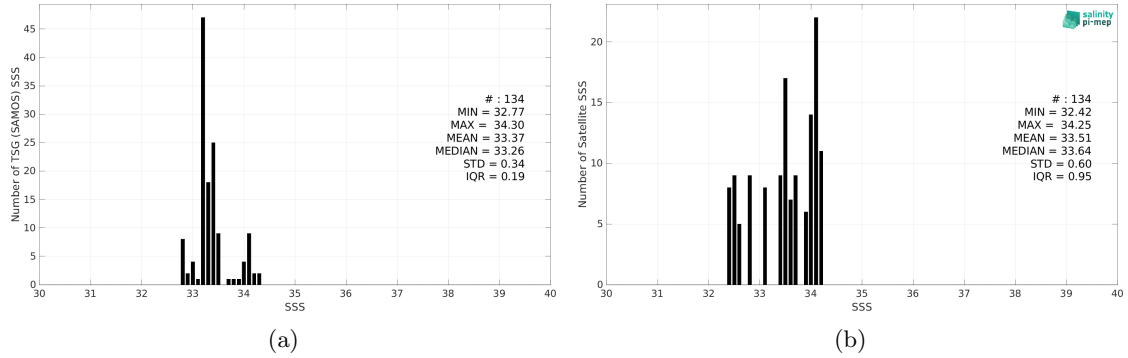
Figure 2: Histograms of SSS from TSG (SAMOS) (a) and SMOS SSS L3 v8 - 18 Days (CATDS-CEC-LOCEAN) (b) considering all match-up pairs per bins of 0.1 over the Ganga and Brahmaputra river plumes Pi-MEP region and for the full satellite product period.
