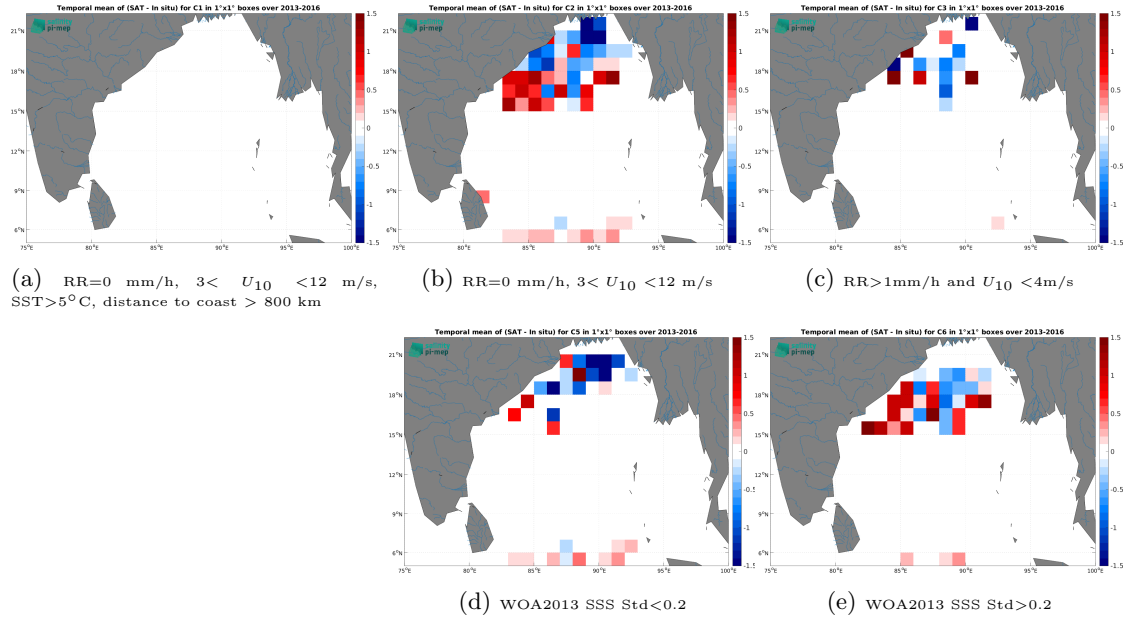
Figure 11: Temporal mean gridded over spatial boxes of size 1^{\circ}\times 1^{\circ} of \Delta\text{SSS} (SMOS SSS L3 v8 - 18 Days (CATDS-CEC-LOCEAN) - Surface drifters) for 5 different subdatasets corresponding to:RR=0 mm/h, 3 < U_{10} < 12 m/s, SST >5^{\circ}\text{C} , distance to coast > 800 km (a), RR=0 mm/h, 3 < U_{10} < 12 m/s (b), RR >1 mm/h and U_{10} < 4 m/s (c), WOA2013 SSS Std <0.2 (d), WOA2013 SSS Std >0.2 (e).
