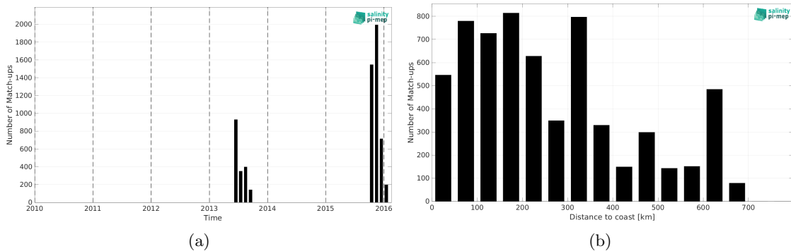
Figure 1: Number of match-ups between Surface drifters and SMOS SSS L3 v8 - 18 Days (CATDS-CEC-LOCEAN) SSS as a function of time (a) and as function of the distance to coast (b) over the Ganga and Brahmaputra river plumes Pi-MEP region and for the full satellite product period.
