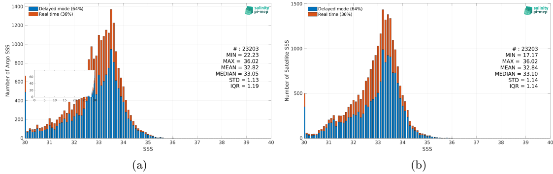
Figure 2: Histograms of SSS from Argo (a) and SMOS SSS L3 v8 - 18 Days (CATDS-CEC-LOCEAN) (b) considering all match-up pairs per bins of 0.1 over the Ganga and Brahmaputra river plumes Pi-MEP region and for the full satellite product period.
