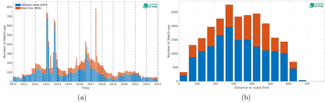
Figure 1: Number of match-ups between Argo and SMOS SSS L3 v8 - 18 Days (CATDS-CEC-LOCEAN) SSS as a function of time (a) and as function of the distance to coast (b) over the Ganga and Brahmaputra river plumes Pi-MEP region and for the full satellite product period.
