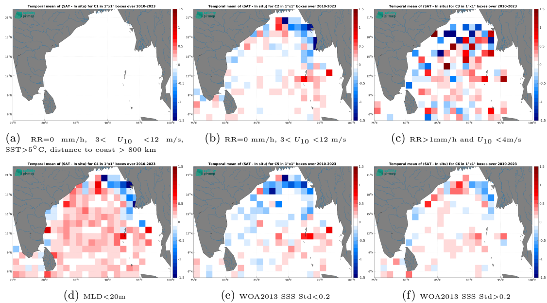
Figure 12: Temporal mean gridded over spatial boxes of size 1^\circ \times 1^\circ of \Delta SSS (SMOS SSS L3 v8 - 18 Days (CATDS-CEC-LOCEAN) - Argo) for 6 different subdatasets corresponding to:RR=0 mm/h, 3 < U_{10} < 12 m/s, SST >5^\circ C, distance to coast > 800 km (a), RR=0 mm/h, 3 < U_{10} < 12 m/s (b), RR >1 mm/h and U_{10} < 4 m/s (c),MLD <20 m (d),WOA2013 SSS Std <0.2 (e),WOA2013 SSS Std >0.2 (f).
