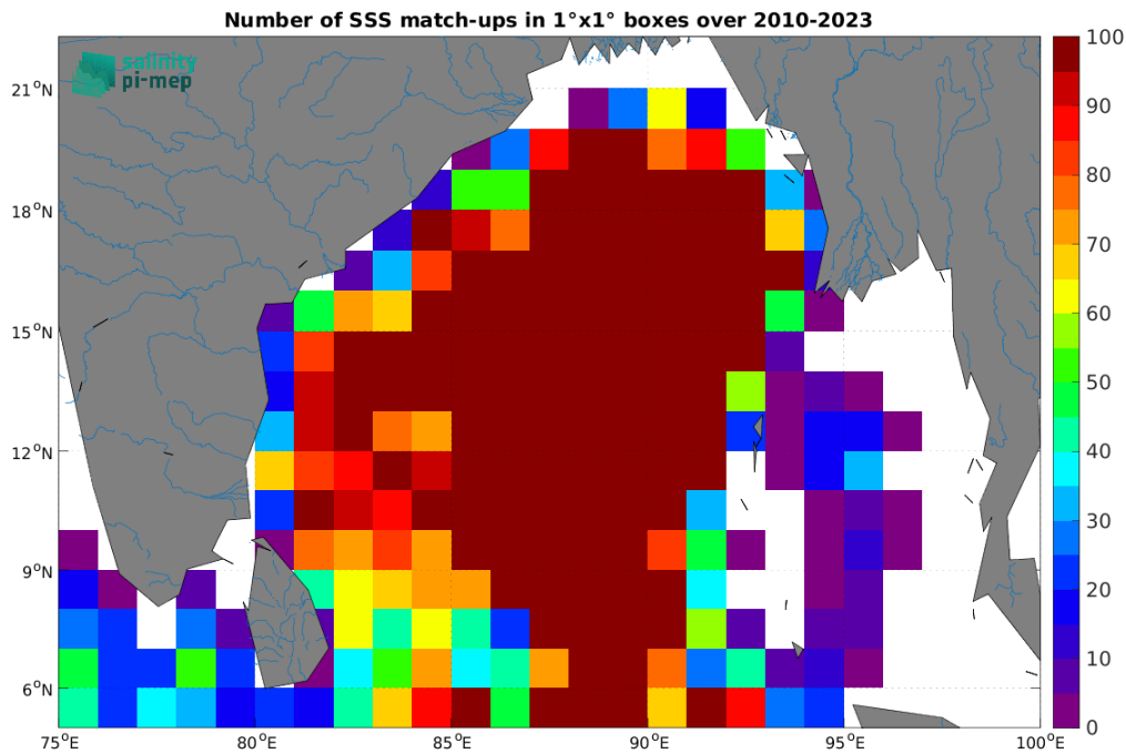
Figure 4: Number of SSS match-ups between Argo SSS and the SMOS SSS L3 v8 - 18 Days (CATDS-CEC-LOCEAN) SSS product for the Ganga and Brahmaputra river plumes Pi-MEP region over 1^\circ \times 1^\circ boxes and for the full satellite product period.
