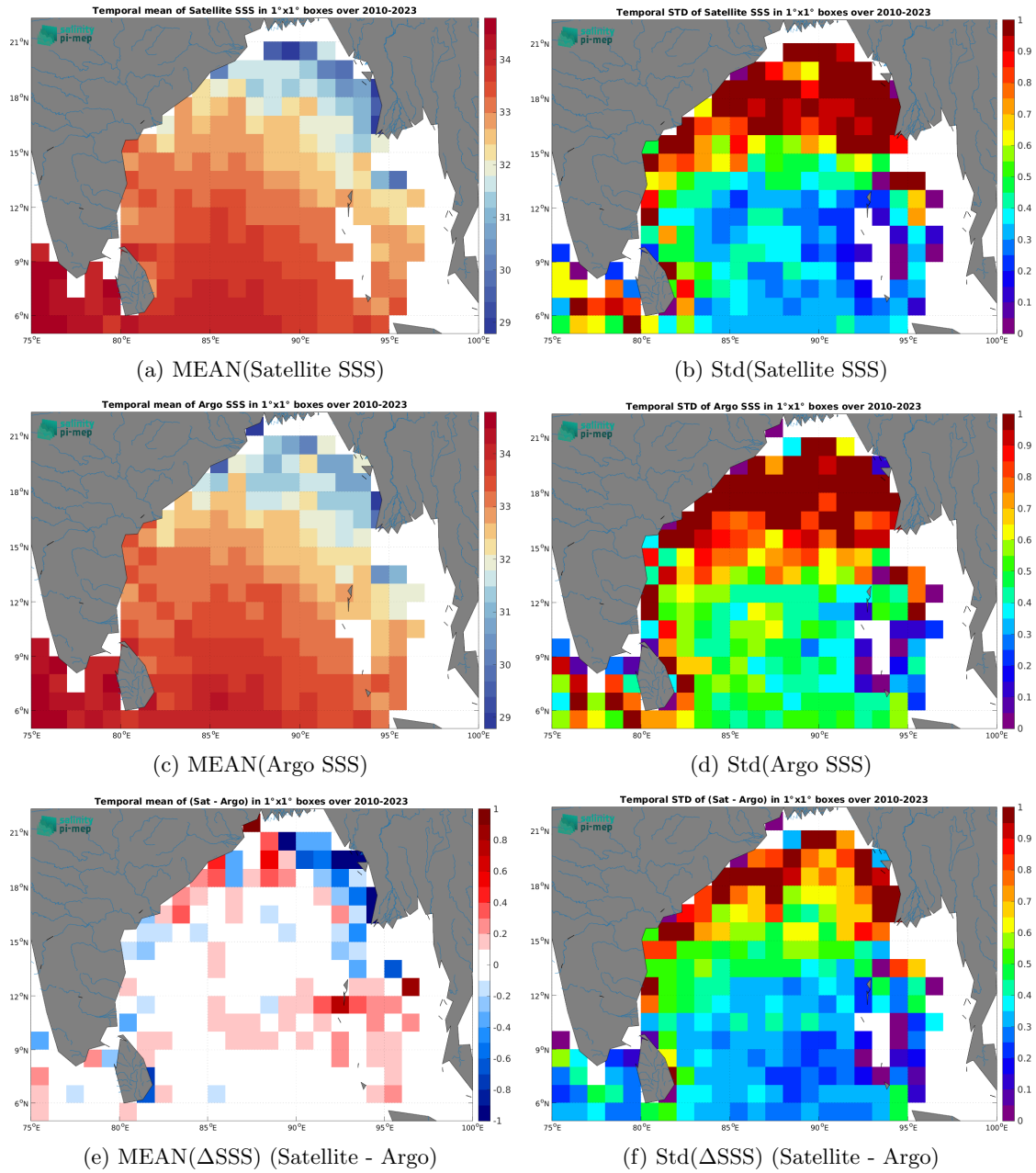
Figure 6: Temporal mean (left) and Std (right) of SSS from SMOS SSS L3 v8 - 18 Days (CATDS-CEC-LOCEAN) (top), Argo (middle), and of \Delta SSS (Satellite - Argo). Only match-up pairs are used to generate these maps.
