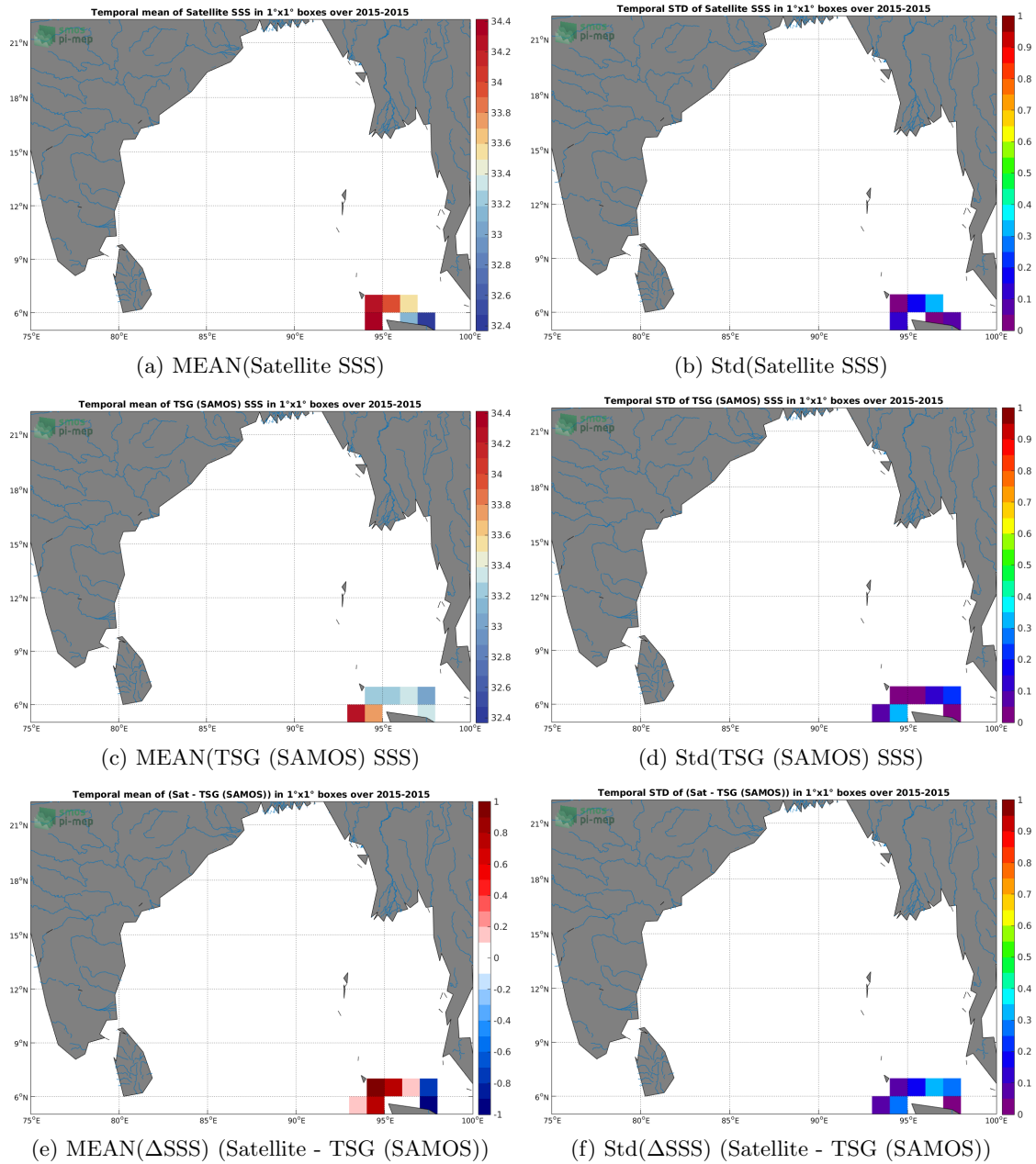
Figure 6: Temporal mean (left) and Std (right) of SSS from SMOS SSS L3 v7 - 9 Days (CATDS-CECOS-LOCEAN) (top), TSG (SAMOS) (middle), and of \Delta SSS (Satellite - TSG (SAMOS)). Only match-up pairs are used to generate these maps.
