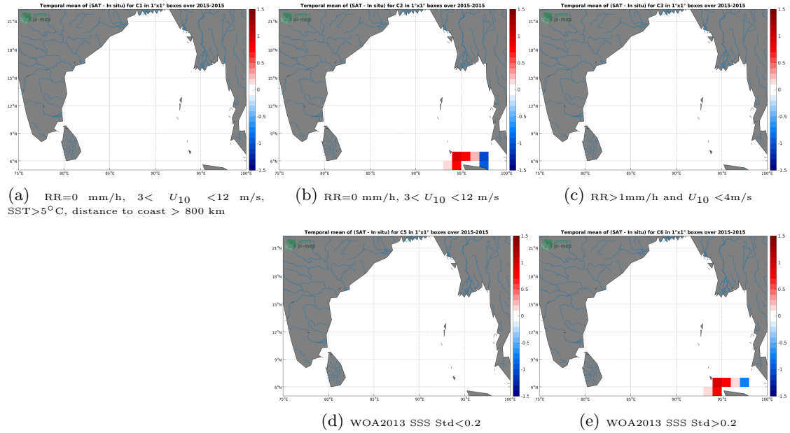
Figure 12: Temporal mean gridded over spatial boxes of size 1^{\circ}\times 1^{\circ} of \Delta\text{SSS} (SMOS SSS L3 v7 - 9 Days (CATDS-CECOS-LOCEAN) - TSG (SAMOS)) for 5 different subdatasets corresponding to:RR=0 mm/h, 3 < U_{10} < 12 m/s, SST > 5^{\circ}\text{C} , distance to coast > 800 km (a), RR=0 mm/h, 3 < U_{10} < 12 m/s (b), RR > 1 mm/h and U_{10} < 4 m/s (c), WOA2013 SSS Std < 0.2 (d), WOA2013 SSS Std > 0.2 (e).
