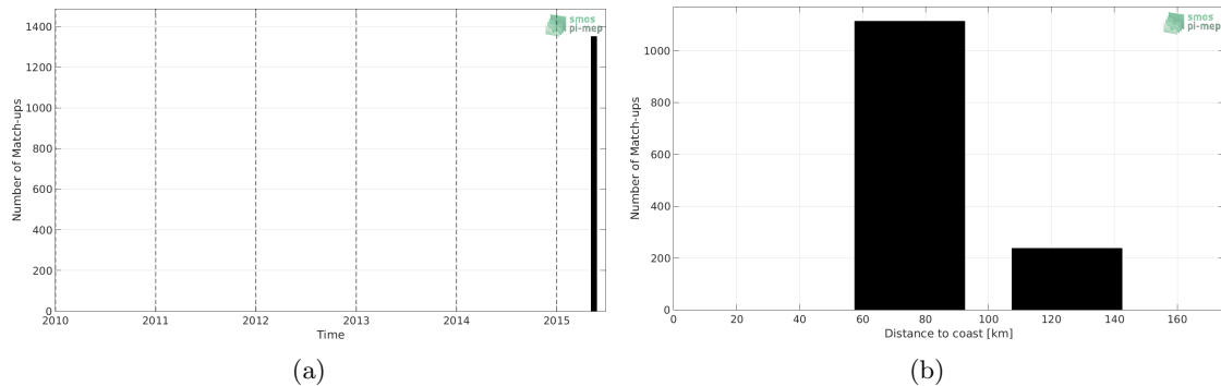
Figure 1: Number of match-ups between TSG (SAMOS) and SMOS SSS L3 v7 - 9 Days (CATDS-CECOS-LOCEAN) SSS as a function of time (a) and as function of the distance to coast (b) over the Ganga and Brahmaputra river plumes Pi-MEP region and for the full satellite product period.
