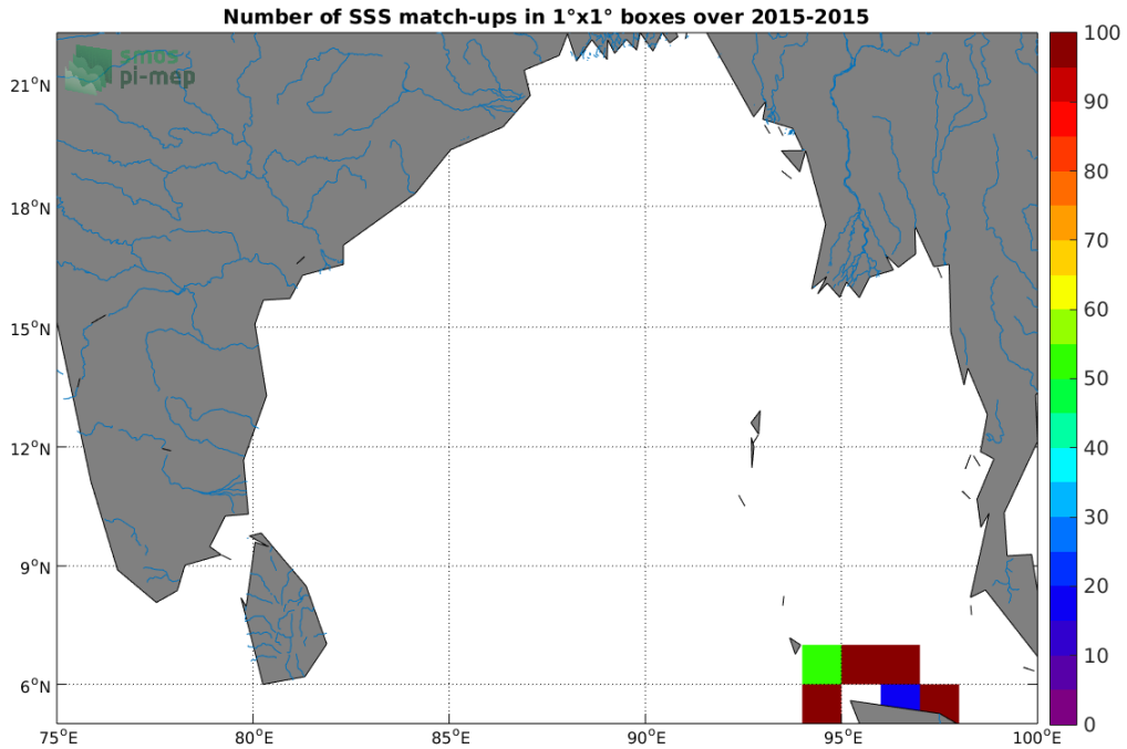
Figure 4: Number of SSS match-ups between TSG (SAMOS) SSS and the SMOS SSS L3 v7 - 9 Days (CATDS-CECOS-LOCEAN) SSS product for the Ganga and Brahmaputra river plumes Pi-MEP region over 1°x1° boxes and for the full satellite product period.
