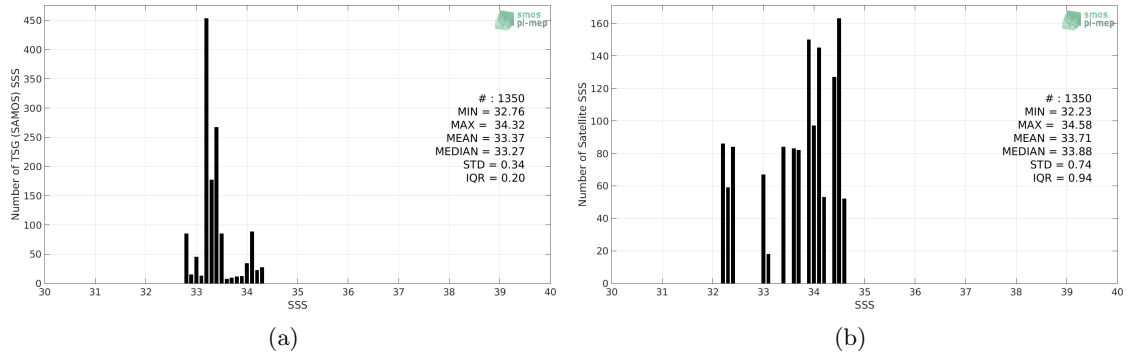
Figure 2: Histograms of SSS from TSG (SAMOS) (a) and SMOS SSS L3 v7 - 9 Days (CATDS-CECOS-LOCEAN) (b) considering all match-up pairs per bins of 0.1 over the Ganga and Brahmaputra river plumes Pi-MEP region and for the full satellite product period.
