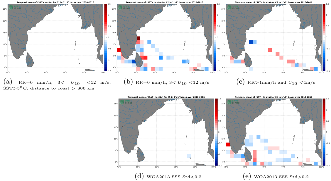
Figure 12: Temporal mean gridded over spatial boxes of size 1^{\circ}\times 1^{\circ} of \Delta\text{SSS} (SMOS SSS L3 v7 - 9 Days (CATDS-CECOS-LOCEAN) - TSG (LEGOS-DM)) for 5 different subdatasets corresponding to:RR=0 mm/h, 3 < U_{10} < 12 m/s, SST > 5^{\circ}\text{C} , distance to coast > 800 km (a), RR=0 mm/h, 3 < U_{10} < 12 m/s (b), RR > 1 mm/h and U_{10} < 4 m/s (c), WOA2013 SSS Std < 0.2 (d), WOA2013 SSS Std > 0.2 (e).
