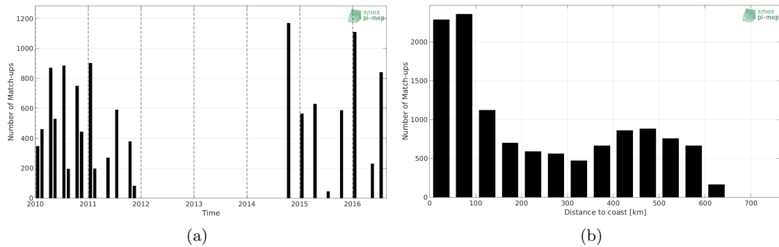
Figure 1: Number of match-ups between TSG (LEGOS-DM) and SMOS SSS L3 v7 - 9 Days (CATDS-CECOS-LOCEAN) SSS as a function of time (a) and as function of the distance to coast (b) over the Ganga and Brahmaputra river plumes Pi-MEP region and for the full satellite product period.
