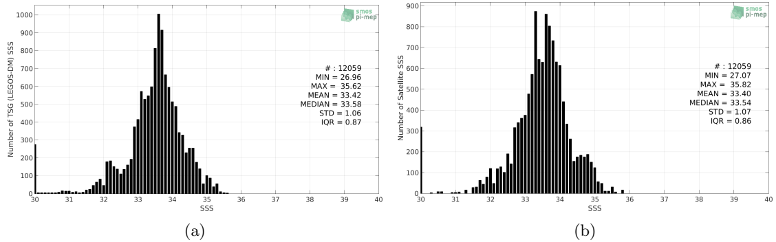
Figure 2: Histograms of SSS from TSG (LEGOS-DM) (a) and SMOS SSS L3 v7 - 9 Days (CATDS-CECOS-LOCEAN) (b) considering all match-up pairs per bins of 0.1 over the Ganga and Brahmaputra river plumes Pi-MEP region and for the full satellite product period.
