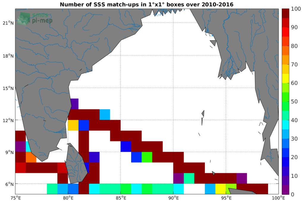
Figure 4: Number of SSS match-ups between TSG (LEGOS-DM) SSS and the SMOS SSS L3 v7 - 9 Days (CATDS-CECOS-LOCEAN) SSS product for the Ganga and Brahmaputra river plumes Pi-MEP region over 1^\circ \times 1^\circ boxes and for the full satellite product period.
