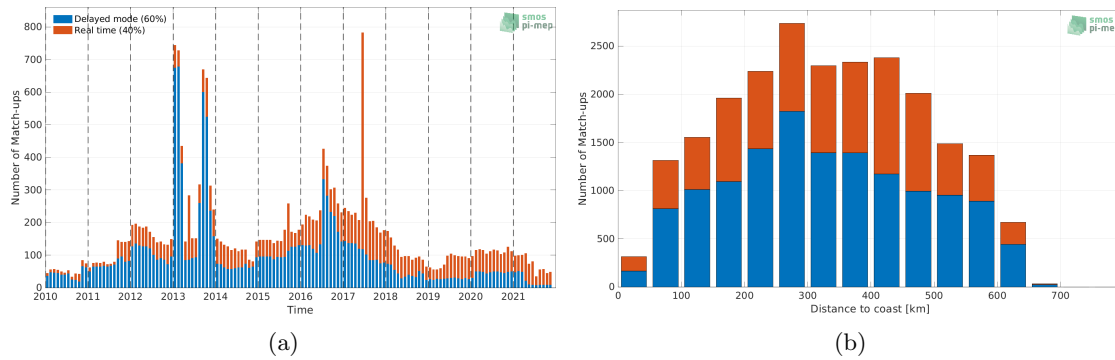
Figure 1: Number of match-ups between Argo and SMOS SSS L3 v7 - 9 Days (CATDS-CECOS-LOCEAN) SSS as a function of time (a) and as function of the distance to coast (b) over the Ganga and Brahmaputra river plumes Pi-MEP region and for the full satellite product period.
