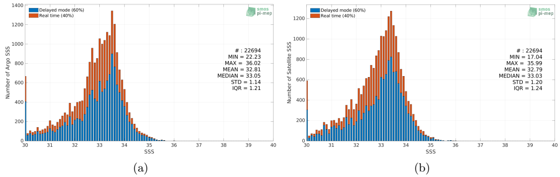
Figure 2: Histograms of SSS from Argo (a) and SMOS SSS L3 v7 - 9 Days (CATDS-CECOS-LOCEAN) (b) considering all match-up pairs per bins of 0.1 over the Ganga and Brahmaputra river plumes Pi-MEP region and for the full satellite product period.
