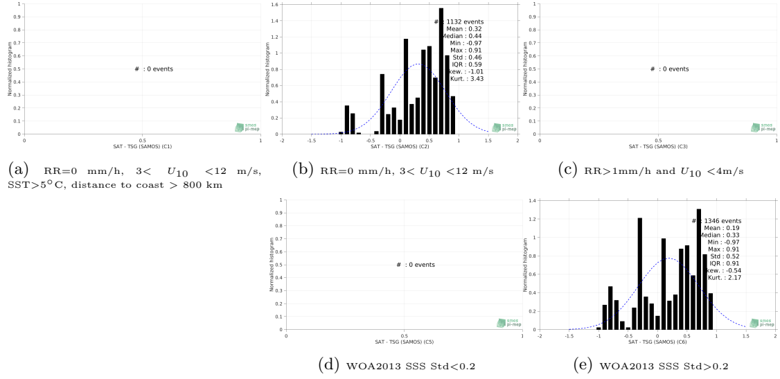
Figure 13: Normalized histogram of \Delta\text{SSS} (SMOS SSS L3 v7 - 18 Days (CATDS-CECOS-LOCEAN) - TSG (SAMOS)) for 5 different subdatasets corresponding to: RR=0 mm/h, 3 < U_{10} < 12 m/s, SST > 5^\circ\text{C} , distance to coast > 800 km (a), RR=0 mm/h, 3 < U_{10} < 12 m/s (b), RR > 1 mm/h and U_{10} < 4 m/s (c), WOA2013 SSS Std < 0.2 (d), WOA2013 SSS Std > 0.2 (e).
