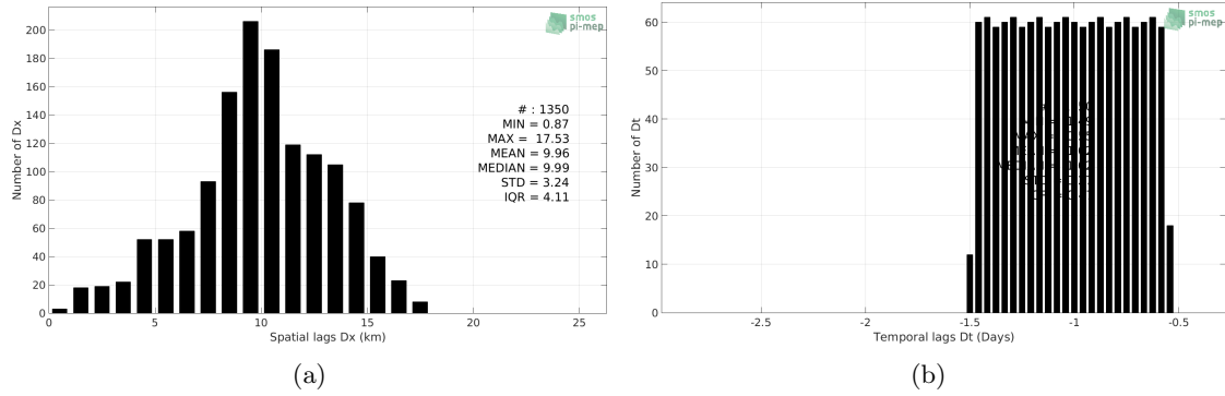
Figure 5: Histograms of the spatial (a) and temporal (b) lags between the location/time of the TSG (SAMOS) measurement and the date of the corresponding SMOS SSS L3 v7 - 18 Days (CATDS-CECOS-LOCEAN) SSS pixel.
