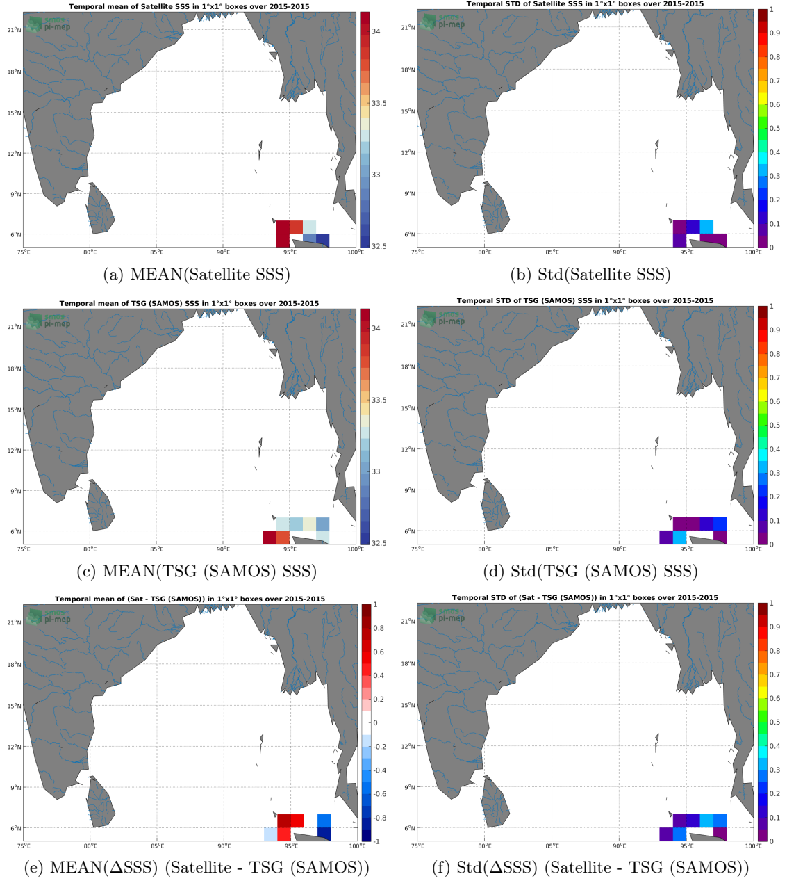
Figure 6: Temporal mean (left) and Std (right) of SSS from SMOS SSS L3 v7 - 18 Days (CATDS-CECOS-LOCEAN) (top), TSG (SAMOS) (middle), and of \Delta SSS (Satellite - TSG (SAMOS)). Only match-up pairs are used to generate these maps.
