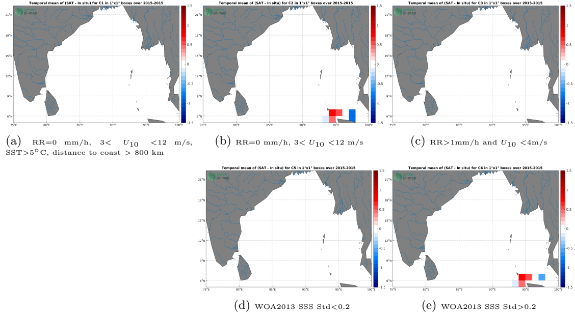
Figure 12: Temporal mean gridded over spatial boxes of size 1^{\circ}\times 1^{\circ} of \Delta\text{SSS} (SMOS SSS L3 v7 - 18 Days (CATDS-CECOS-LOCEAN) - TSG (SAMOS)) for 5 different subdatasets corresponding to:RR=0 mm/h, 3 < U_{10} < 12 m/s, SST >5^{\circ}\text{C} , distance to coast > 800 km (a), RR=0 mm/h, 3 < U_{10} < 12 m/s (b), RR >1 mm/h and U_{10} < 4 m/s (c), WOA2013 SSS Std <0.2 (d), WOA2013 SSS Std >0.2 (e).
