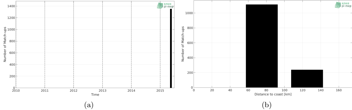
Figure 1: Number of match-ups between TSG (SAMOS) and SMOS SSS L3 v7 - 18 Days (CATDS-CECOS-LOCEAN) SSS as a function of time (a) and as function of the distance to coast (b) over the Ganga and Brahmaputra river plumes Pi-MEP region and for the full satellite product period.
