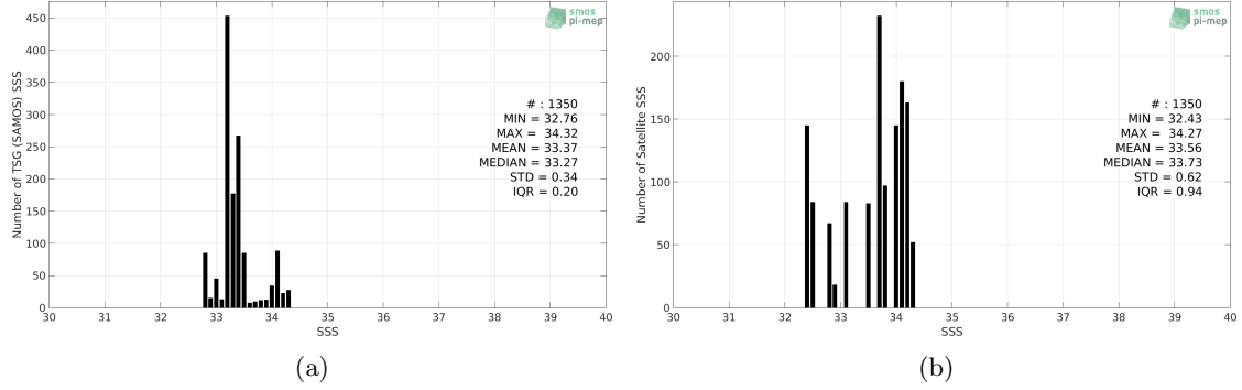
Figure 2: Histograms of SSS from TSG (SAMOS) (a) and SMOS SSS L3 v7 - 18 Days (CATDS-CECOS-LOCEAN) (b) considering all match-up pairs per bins of 0.1 over the Ganga and Brahmaputra river plumes Pi-MEP region and for the full satellite product period.
