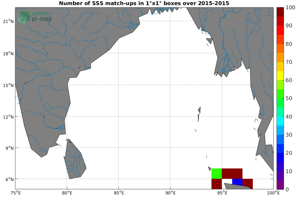
Figure 4: Number of SSS match-ups between TSG (SAMOS) SSS and the SMOS SSS L3 v7 - 18 Days (CATDS-CECOS-LOCEAN) SSS product for the Ganga and Brahmaputra river plumes Pi-MEP region over 1^\circ \times 1^\circ boxes and for the full satellite product period.
