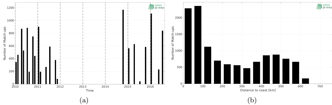
Figure 1: Number of match-ups between TSG (LEGOS-DM) and SMOS SSS L3 v7 - 18 Days (CATDS-CECOS-LOCEAN) SSS as a function of time (a) and as function of the distance to coast (b) over the Ganga and Brahmaputra river plumes Pi-MEP region and for the full satellite product period.
