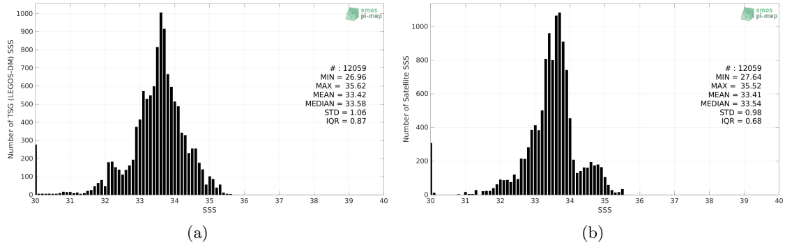
Figure 2: Histograms of SSS from TSG (LEGOS-DM) (a) and SMOS SSS L3 v7 - 18 Days (CATDS-CECOS-LOCEAN) (b) considering all match-up pairs per bins of 0.1 over the Ganga and Brahmaputra river plumes Pi-MEP region and for the full satellite product period.
