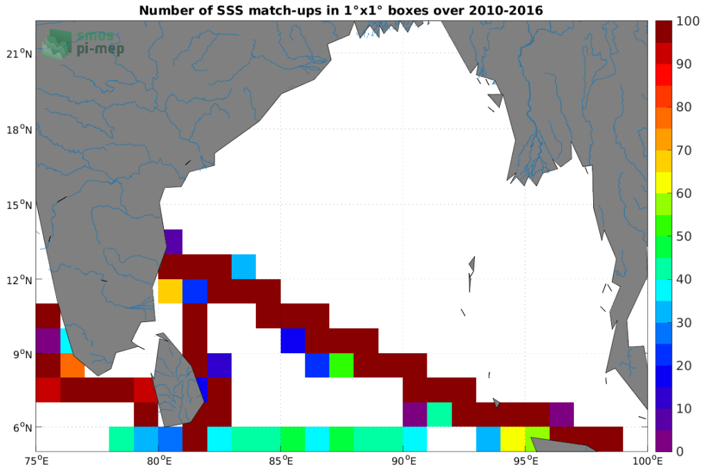
Figure 4: Number of SSS match-ups between TSG (LEGOS-DM) SSS and the SMOS SSS L3 v7 - 18 Days (CATDS-CECOS-LOCEAN) SSS product for the Ganga and Brahmaputra river plumes Pi-MEP region over 1^\circ \times 1^\circ boxes and for the full satellite product period.
