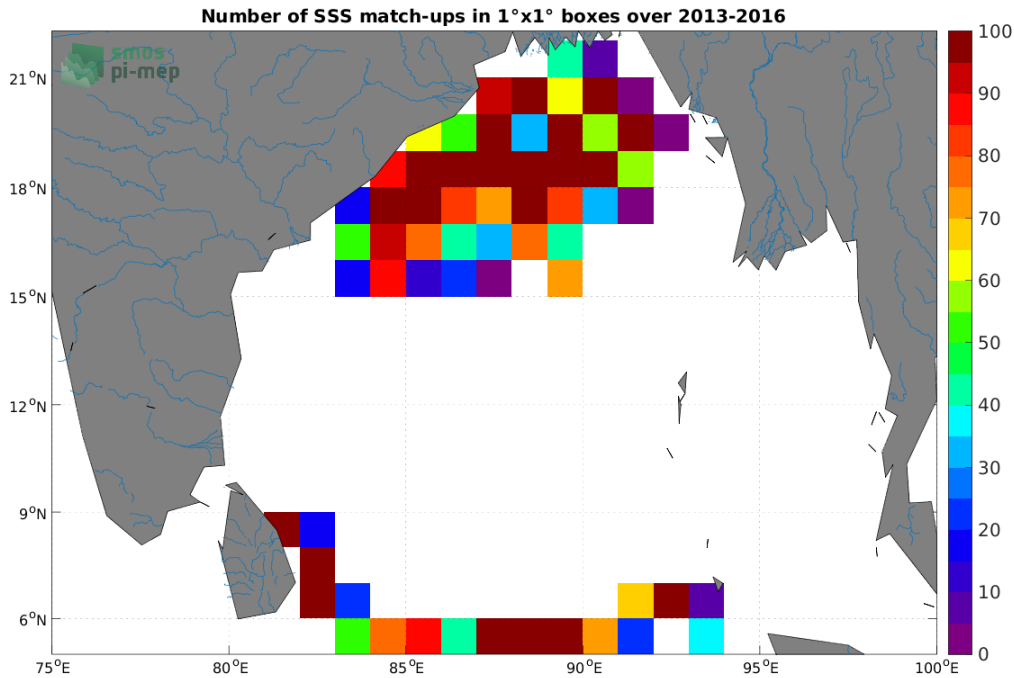
Figure 3: Number of SSS match-ups between Surface drifters SSS and the SMOS SSS L3 v7 - 18 Days (CATDS-CECOS-LOCEAN) SSS product for the Ganga and Brahmaputra river plumes Pi-MEP region over 1^\circ \times 1^\circ boxes and for the full satellite product period.
