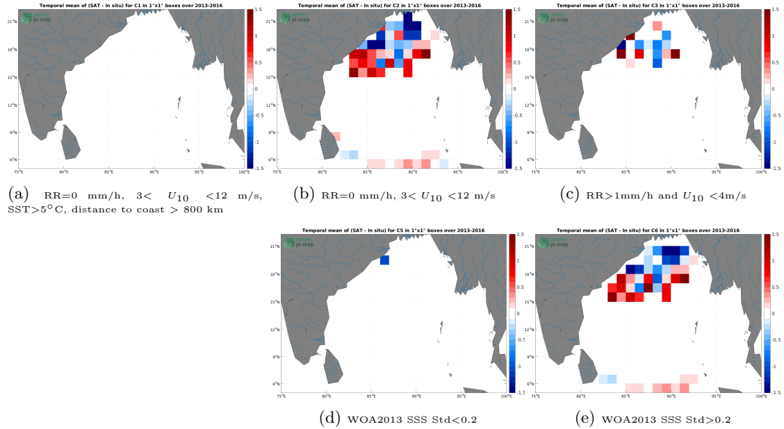
Figure 11: Temporal mean gridded over spatial boxes of size 1^{\circ}\times 1^{\circ} of \Delta\text{SSS} (SMOS SSS L3 v7 - 18 Days (CATDS-CECOS-LOCEAN) - Surface drifters) for 5 different subdatasets corresponding to:RR=0 mm/h, 3 < U_{10} < 12 m/s, SST >5^{\circ}\text{C} , distance to coast > 800 km (a), RR=0 mm/h, 3 < U_{10} < 12 m/s (b), RR >1 mm/h and U_{10} < 4 m/s (c), WOA2013 SSS Std <0.2 (d), WOA2013 SSS Std >0.2 (e).
