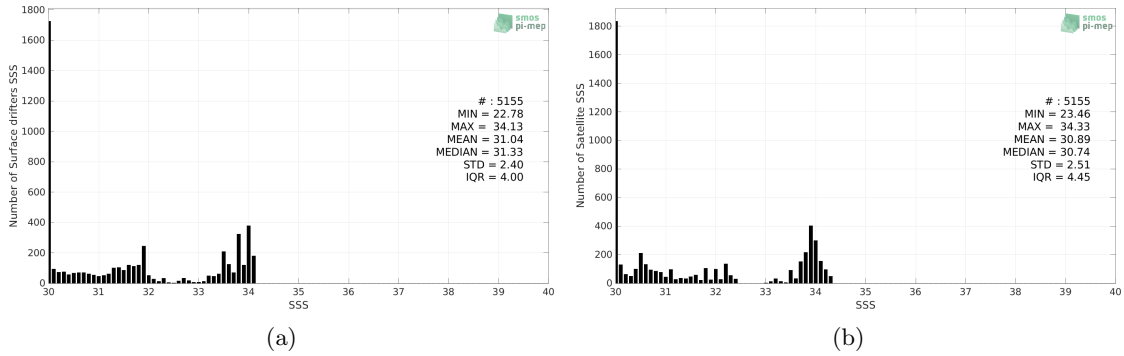
Figure 2: Histograms of SSS from Surface drifters (a) and SMOS SSS L3 v7 - 18 Days (CATDS-CECOS-LOCEAN) (b) considering all match-up pairs per bins of 0.1 over the Ganga and Brahmaputra river plumes Pi-MEP region and for the full satellite product period.
