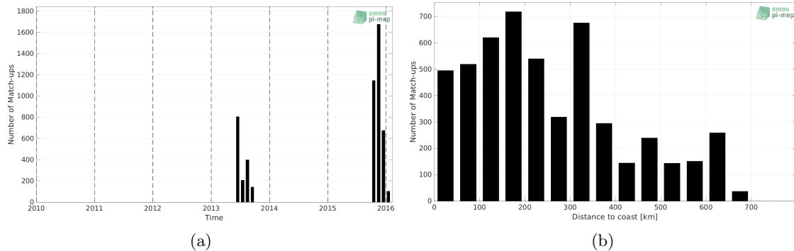
Figure 1: Number of match-ups between Surface drifters and SMOS SSS L3 v7 - 18 Days (CATDS-CECOS-LOCEAN) SSS as a function of time (a) and as function of the distance to coast (b) over the Ganga and Brahmaputra river plumes Pi-MEP region and for the full satellite product period.
