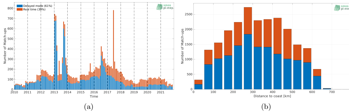
Figure 1: Number of match-ups between Argo and SMOS SSS L3 v7 - 18 Days (CATDS-CECOS-LOCEAN) SSS as a function of time (a) and as function of the distance to coast (b) over the Ganga and Brahmaputra river plumes Pi-MEP region and for the full satellite product period.
