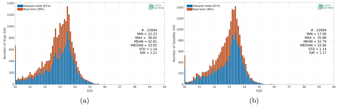
Figure 2: Histograms of SSS from Argo (a) and SMOS SSS L3 v7 - 18 Days (CATDS-CECOS-LOCEAN) (b) considering all match-up pairs per bins of 0.1 over the Ganga and Brahmaputra river plumes Pi-MEP region and for the full satellite product period.
