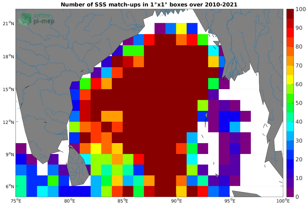
Figure 4: Number of SSS match-ups between Argo SSS and the SMOS SSS L3 v7 - 18 Days (CATDS-CECOS-LOCEAN) SSS product for the Ganga and Brahmaputra river plumes Pi-MEP region over 1^\circ \times 1^\circ boxes and for the full satellite product period.
