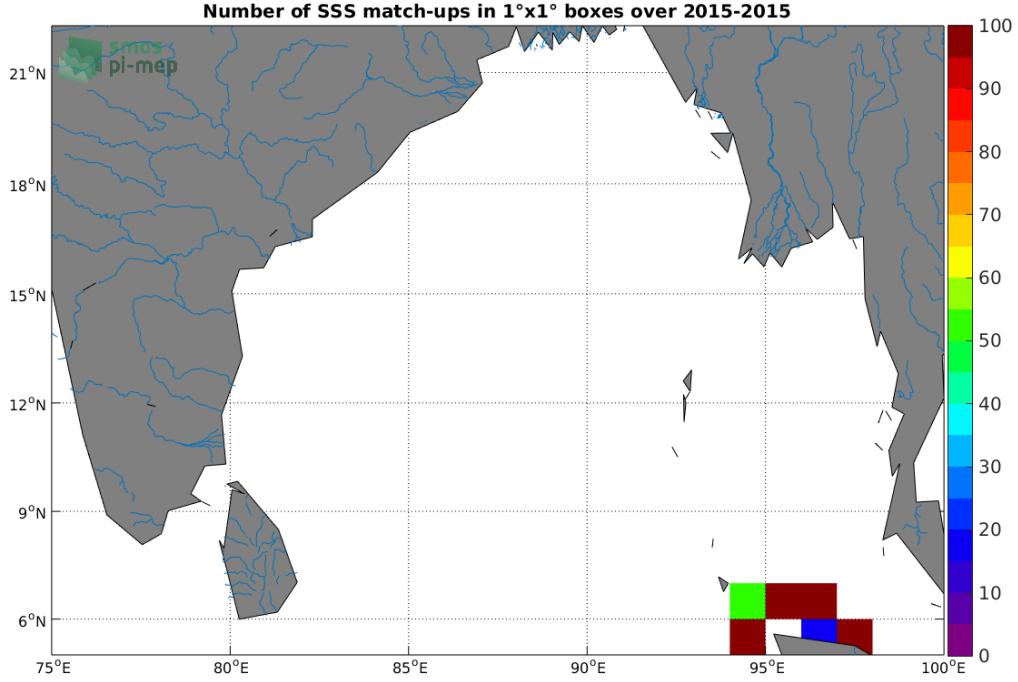
Figure 4: Number of SSS match-ups between TSG (SAMOS) SSS and the SMOS SSS L3 v5 - 9 Days (CATDS-CECOS-LOCEAN) SSS product for the Ganga and Brahmaputra river plumes Pi-MEP region over 1^\circ \times 1^\circ boxes and for the full satellite product period.
