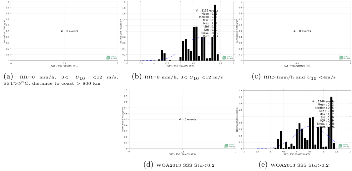
Figure 13: Normalized histogram of \Delta\text{SSS} (SMOS SSS L3 v5 - 9 Days (CATDS-CECOS-LOCEAN) - TSG (SAMOS)) for 5 different subdatasets corresponding to: RR=0 mm/h, 3 < U_{10} < 12 m/s, SST > 5^\circ\text{C} , distance to coast > 800 km (a), RR=0 mm/h, 3 < U_{10} < 12 m/s (b), RR > 1\text{mm/h} and U_{10} < 4\text{m/s} (c), WOA2013 SSS Std < 0.2 (d), WOA2013 SSS Std > 0.2 (e).
