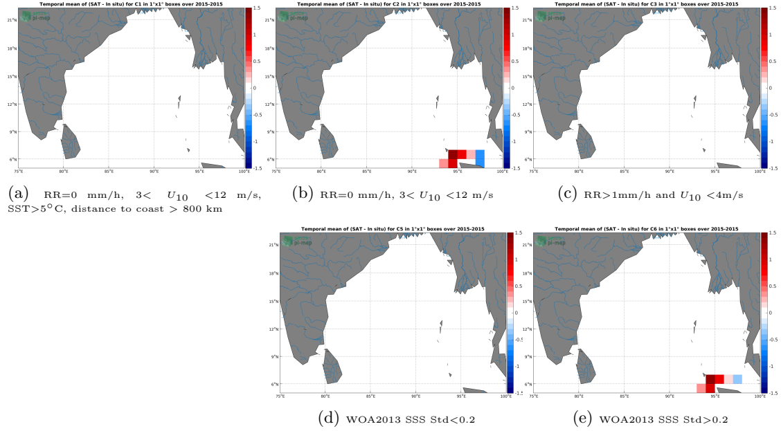
Figure 12: Temporal mean gridded over spatial boxes of size 1^{\circ} \times 1^{\circ} of \Delta\text{SSS} (SMOS SSS L3 v5 - 9 Days (CATDS-CECOS-LOCEAN) - TSG (SAMOS)) for 5 different subdatasets corresponding to:RR=0 mm/h, 3 < U_{10} < 12 m/s, SST >5^{\circ}\text{C} , distance to coast > 800 km (a), RR=0 mm/h, 3 < U_{10} < 12 m/s (b), RR >1 mm/h and U_{10} < 4 m/s (c), WOA2013 SSS Std <0.2 (d), WOA2013 SSS Std >0.2 (e).
