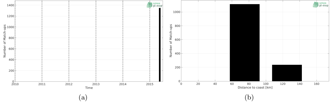
Figure 1: Number of match-ups between TSG (SAMOS) and SMOS SSS L3 v5 - 9 Days (CATDS-CECOS-LOCEAN) SSS as a function of time (a) and as function of the distance to coast (b) over the Ganga and Brahmaputra river plumes Pi-MEP region and for the full satellite product period.
