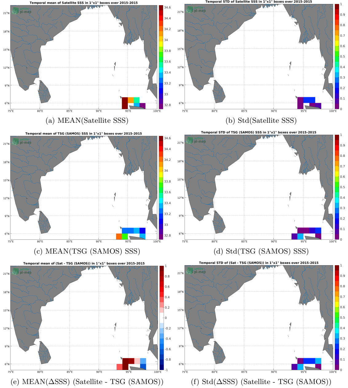
Figure 6: Temporal mean (left) and Std (right) of SSS from SMOS SSS L3 v5 - 9 Days (CATDS-CECOS-LOCEAN) (top), TSG (SAMOS) (middle), and of \Delta SSS (Satellite - TSG (SAMOS)). Only match-up pairs are used to generate these maps.
