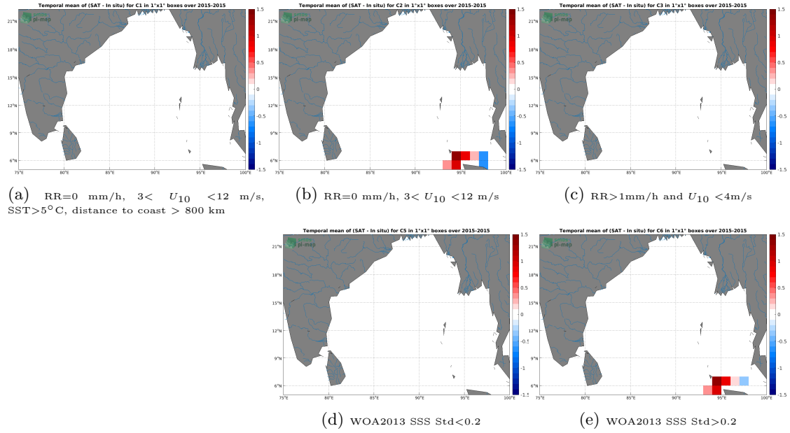
Figure 12: Temporal mean gridded over spatial boxes of size 1^{\circ}\times 1^{\circ} of \Delta\text{SSS} (SMOS SSS L3 v5 - 9 Days (CATDS-CECOS-LOCEAN) - TSG (SAMOS)) for 5 different subdatasets corresponding to:RR=0 mm/h, 3 < U_{10} < 12 m/s, SST >5^{\circ}\text{C} , distance to coast > 800 km (a), RR=0 mm/h, 3 < U_{10} < 12 m/s (b), RR >1 mm/h and U_{10} < 4 m/s (c), WOA2013 SSS Std <0.2 (d), WOA2013 SSS Std >0.2 (e).
