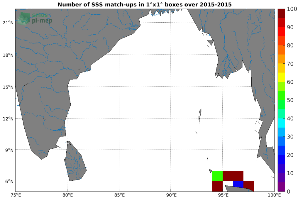
Figure 4: Number of SSS match-ups between TSG (SAMOS) SSS and the SMOS SSS L3 v5 - 9 Days (CATDS-CECOS-LOCEAN) SSS product for the Ganga and Brahmaputra river plumes Pi-MEP region over 1°x1° boxes and for the full satellite product period.
