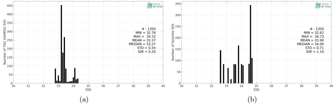
Figure 2: Histograms of SSS from TSG (SAMOS) (a) and SMOS SSS L3 v5 - 9 Days (CATDS-CECOS-LOCEAN) (b) considering all match-up pairs per bins of 0.1 over the Ganga and Brahmaputra river plumes Pi-MEP region and for the full satellite product period.
