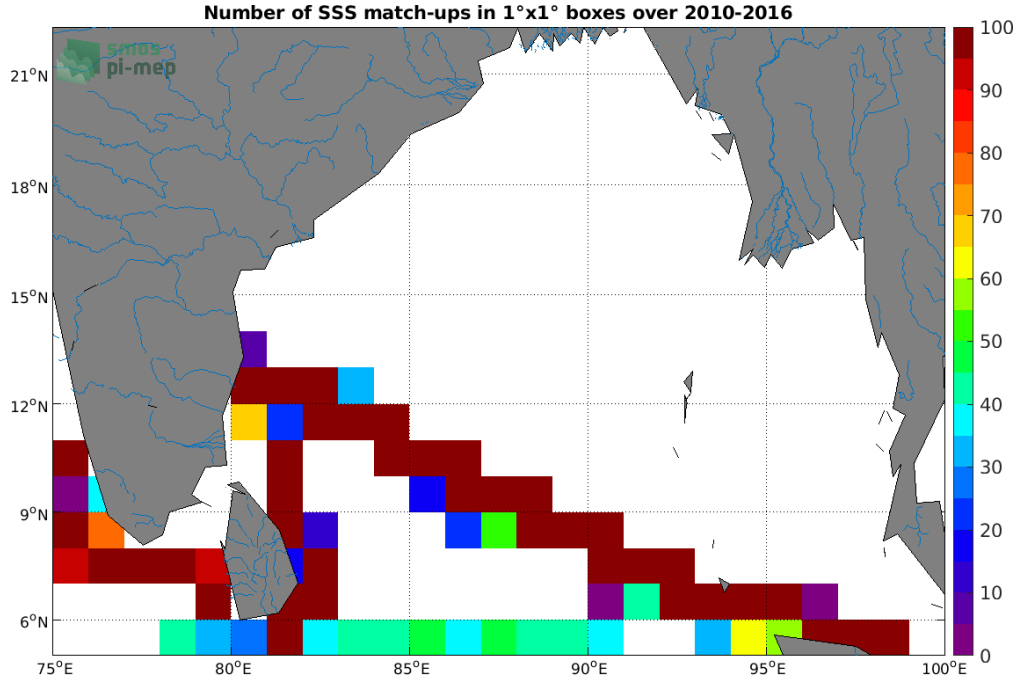
Figure 4: Number of SSS match-ups between TSG (LEGOS-DM) SSS and the SMOS SSS L3 v5 - 9 Days (CATDS-CECOS-LOCEAN) SSS product for the Ganga and Brahmaputra river plumes Pi-MEP region over 1^\circ \times 1^\circ boxes and for the full satellite product period.
