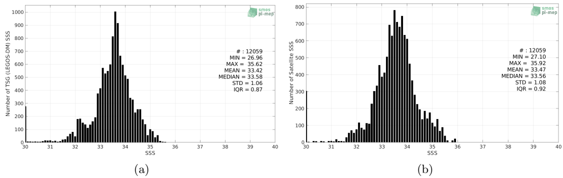
Figure 2: Histograms of SSS from TSG (LEGOS-DM) (a) and SMOS SSS L3 v5 - 9 Days (CATDS-CECOS-LOCEAN) (b) considering all match-up pairs per bins of 0.1 over the Ganga and Brahmaputra river plumes Pi-MEP region and for the full satellite product period.
