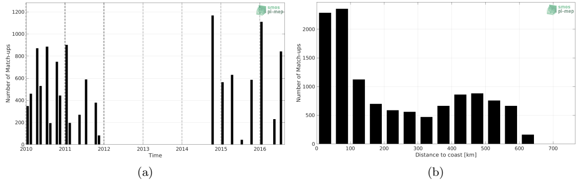
Figure 1: Number of match-ups between TSG (LEGOS-DM) and SMOS SSS L3 v5 - 9 Days (CATDS-CECOS-LOCEAN) SSS as a function of time (a) and as function of the distance to coast (b) over the Ganga and Brahmaputra river plumes Pi-MEP region and for the full satellite product period.
