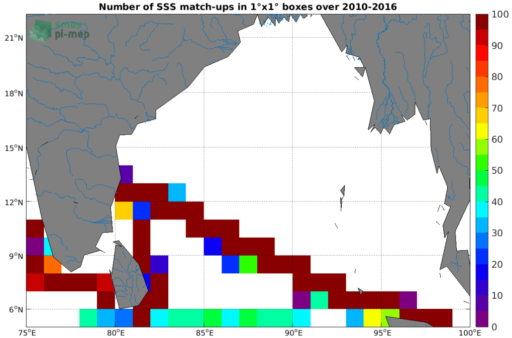
Figure 4: Number of SSS match-ups between TSG (LEGOS-DM) SSS and the SMOS SSS L3 v5 - 9 Days (CATDS-CECOS-LOCEAN) SSS product for the Ganga and Brahmaputra river plumes Pi-MEP region over 1°x1° boxes and for the full satellite product period.
