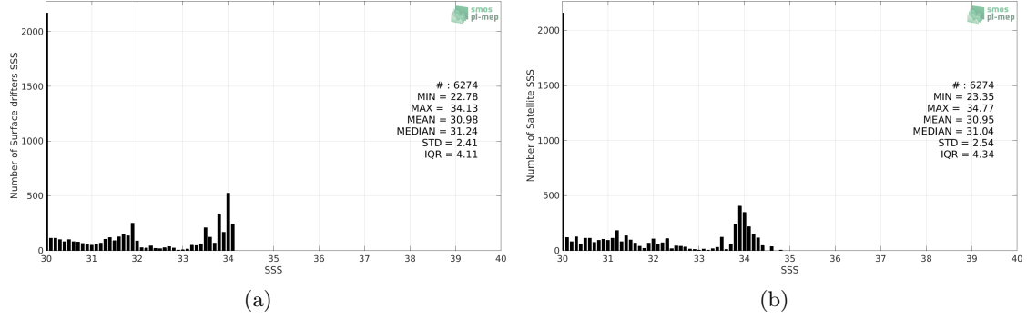
Figure 2: Histograms of SSS from Surface drifters (a) and SMOS SSS L3 v5 - 9 Days (CATDS-CECOS-LOCEAN) (b) considering all match-up pairs per bins of 0.1 over the Ganga and Brahmaputra river plumes Pi-MEP region and for the full satellite product period.
