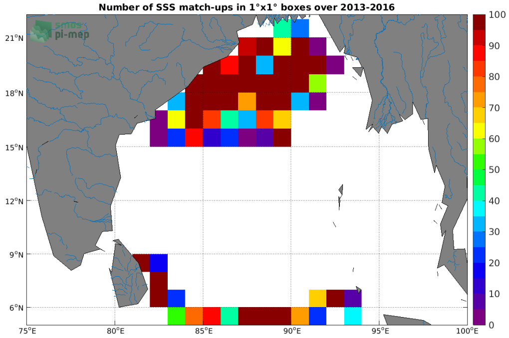
Figure 3: Number of SSS match-ups between Surface drifters SSS and the SMOS SSS L3 v5 - 9 Days (CATDS-CECOS-LOCEAN) SSS product for the Ganga and Brahmaputra river plumes Pi-MEP region over 1^\circ \times 1^\circ boxes and for the full satellite product period.
