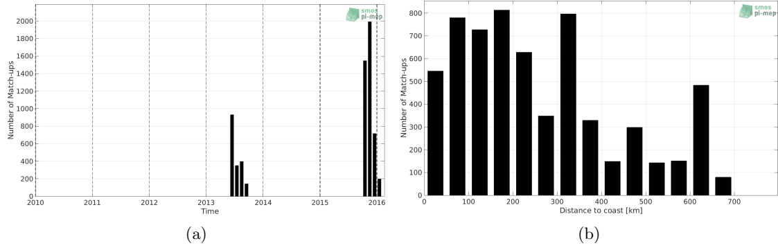
Figure 1: Number of match-ups between Surface drifters and SMOS SSS L3 v5 - 9 Days (CATDS-CECOS-LOCEAN) SSS as a function of time (a) and as function of the distance to coast (b) over the Ganga and Brahmaputra river plumes Pi-MEP region and for the full satellite product period.
