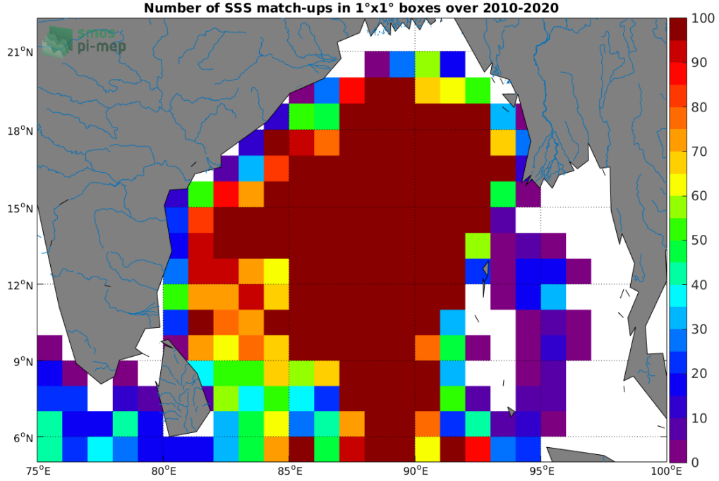
Figure 4: Number of SSS match-ups between Argo SSS and the SMOS SSS L3 v5 - 9 Days (CATDS-CECOS-LOCEAN) SSS product for the Ganga and Brahmaputra river plumes Pi-MEP region over 1^\circ \times 1^\circ boxes and for the full satellite product period.
