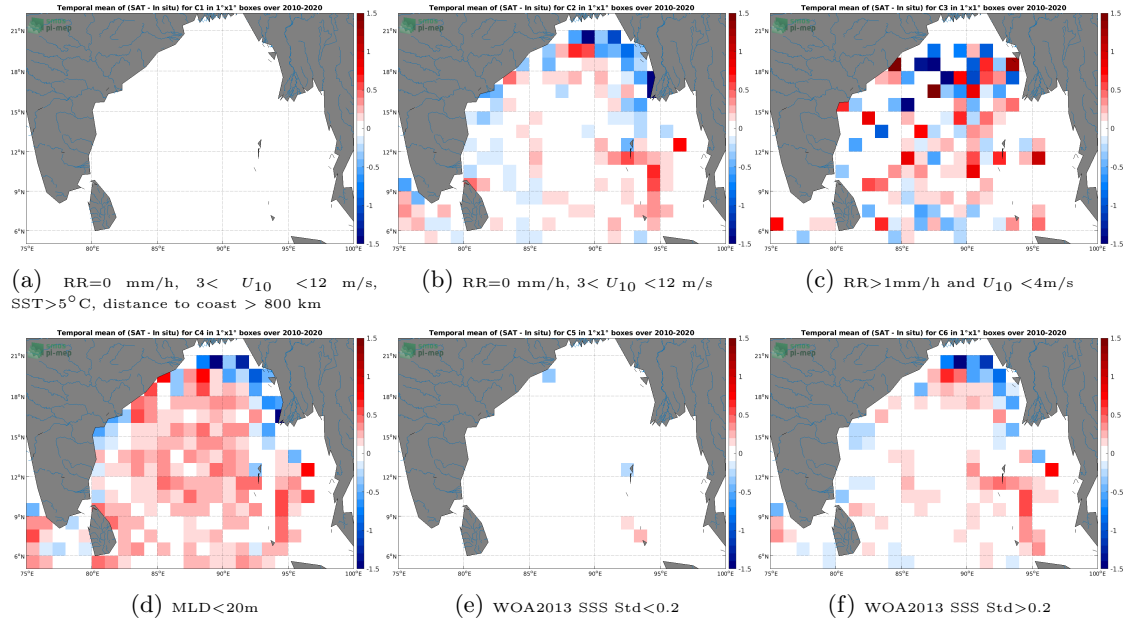
Figure 12: Temporal mean gridded over spatial boxes of size 1^\circ \times 1^\circ of \Delta SSS (SMOS SSS L3 v5 - 9 Days (CATDS-CECOS-LOCEAN) - Argo) for 6 different subdatasets corresponding to: RR=0 mm/h, 3 < U_{10} < 12 m/s, SST > 5^\circ C , distance to coast > 800 km (a), RR=0 mm/h, 3 < U_{10} < 12 m/s (b), RR > 1 mm/h and U_{10} < 4 m/s (c), MLD < 20 m (d), WOA2013 SSS Std < 0.2 (e), WOA2013 SSS Std > 0.2 (f).
