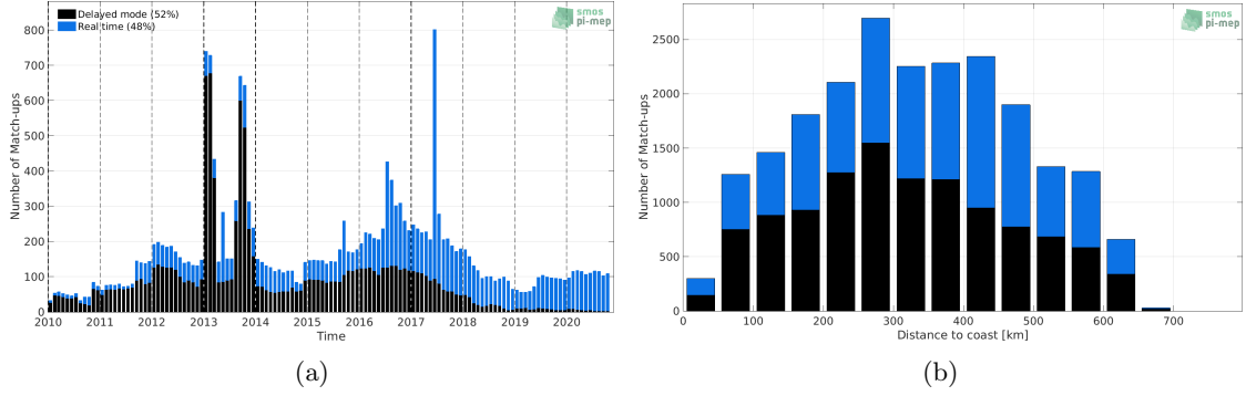
Figure 1: Number of match-ups between Argo and SMOS SSS L3 v5 - 9 Days (CATDS-CECOS-LOCEAN) SSS as a function of time (a) and as function of the distance to coast (b) over the Ganga and Brahmaputra river plumes Pi-MEP region and for the full satellite product period.
