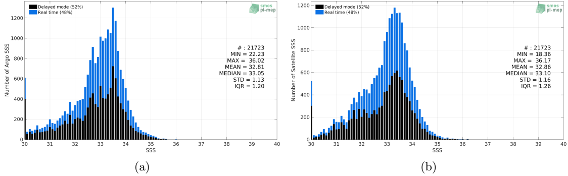
Figure 2: Histograms of SSS from Argo (a) and SMOS SSS L3 v5 - 9 Days (CATDS-CECOS-LOCEAN) (b) considering all match-up pairs per bins of 0.1 over the Ganga and Brahmaputra river plumes Pi-MEP region and for the full satellite product period.
