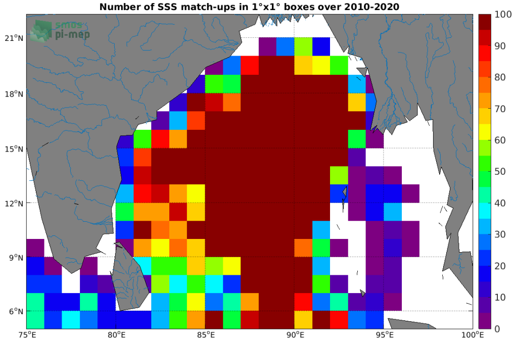
Figure 4: Number of SSS match-ups between Argo SSS and the SMOS SSS L3 v5 - 9 Days (CATDS-CECOS-LOCEAN) SSS product for the Ganga and Brahmaputra river plumes Pi-MEP region over 1°x1° boxes and for the full satellite product period.
